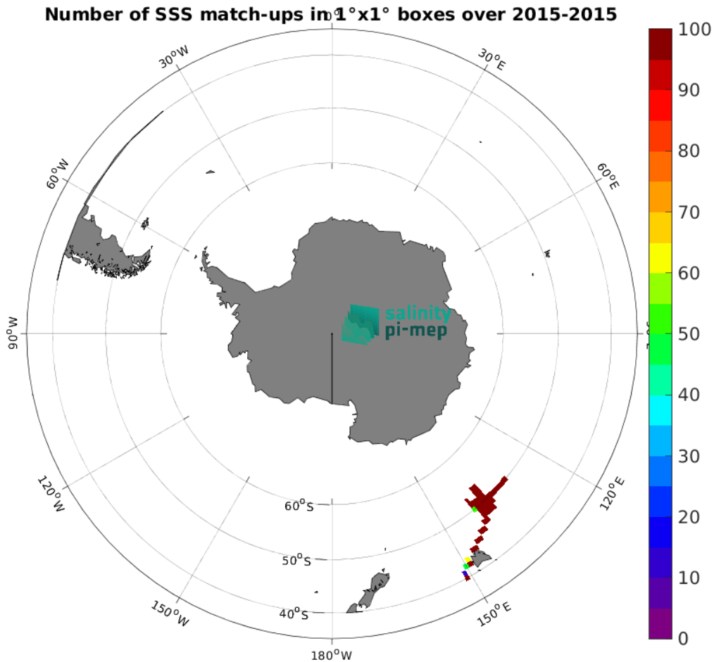
Figure 5: Number of SSS match-ups between TSG (GOSUD-Research-vessel) SSS and the Aquarius SSS L3 OR v5 - Monthly - Rain mask (NASA-GSFC) SSS product for the Roaring Forties and Furious Fifties Pi-MEP region over 1^\circ \times 1^\circ boxes and for the full satellite product period.
