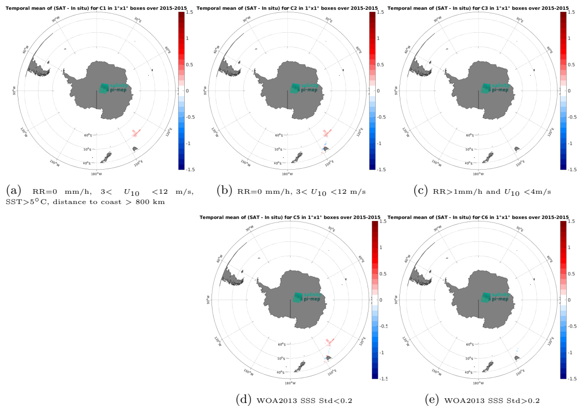
Figure 14: Temporal mean gridded over spatial boxes of size 1^\circ \times 1^\circ of \Delta SSS (Aquarius SSS L3 OR v5 - Monthly - Rain mask (NASA-GSFC) - TSG (GOSUD-Research-vessel)) for 5 different subdatasets corresponding to:RR=0 mm/h, 3 < U_{10} < 12 m/s, SST>5°C, distance to coast > 800 km (a), RR=0 mm/h, 3 < U_{10} < 12 m/s (b), RR>1mm/h and U_{10} < 4 m/s (c), WOA2013 SSS Std<0.2 (d), WOA2013 SSS Std>0.2 (e).
