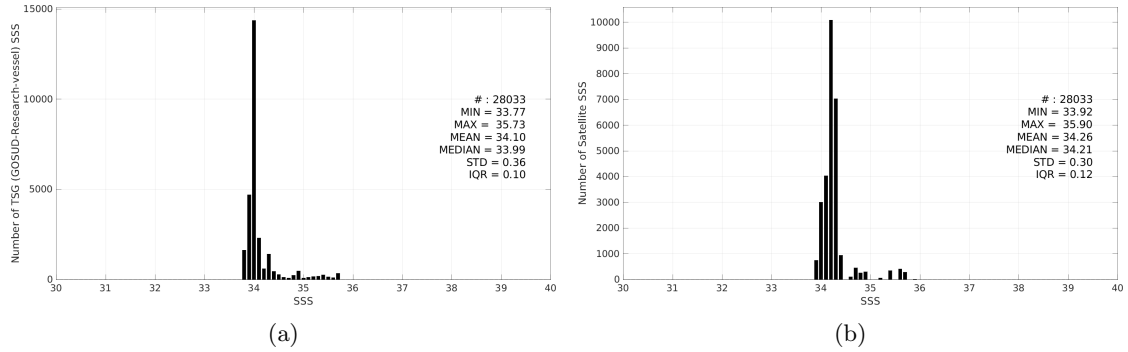
Figure 3: Histograms of SSS from TSG (GOSUD-Research-vessel) (a) and Aquarius SSS L3 OR v5 - Monthly - Rain mask (NASA-GSFC) (b) considering all match-up pairs per bins of 0.1 over the Roaring Forties and Furious Fifties Pi-MEP region and for the full satellite product period.
