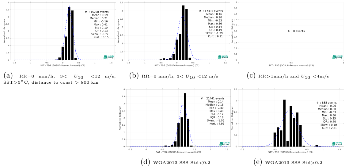
Figure 15: Normalized histogram of \Delta SSS (Aquarius SSS L3 OR v5 - Monthly - Rain mask (NASA-GSFC) - TSG (GOSUD-Research-vessel)) for 5 different subdatasets corresponding to: RR=0 mm/h, 3 < U_{10} < 12 m/s, SST > 5°C, distance to coast > 800 km (a), RR=0 mm/h, 3 < U_{10} < 12 m/s (b), RR > 1mm/h and U_{10} < 4 m/s (c), WOA2013 SSS Std < 0.2 (d), WOA2013 SSS Std > 0.2 (e).
