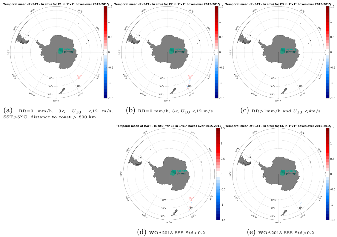
Figure 12: Temporal mean gridded over spatial boxes of size 1^\circ \times 1^\circ of \Delta SSS (Aquarius SSS L3 OR v5 - Monthly - Rain mask (NASA-GSFC) - TSG (GOSUD-Research-vessel)) for 5 different subdatasets corresponding to:RR=0 mm/h, 3 < U_{10} < 12 m/s, SST>5°C, distance to coast > 800 km (a), RR=0 mm/h, 3 < U_{10} < 12 m/s (b), RR>1mm/h and U_{10} < 4 m/s (c), WOA2013 SSS Std<0.2 (d), WOA2013 SSS Std>0.2 (e).
