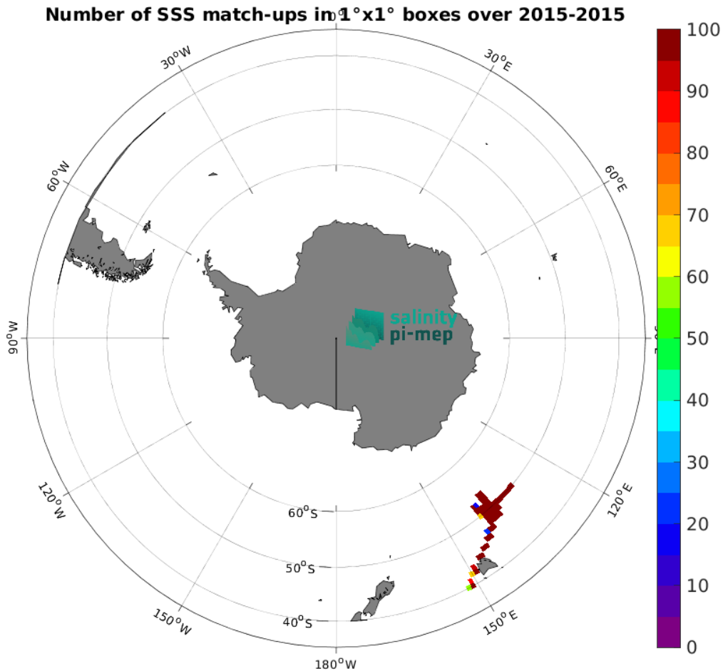
Figure 4: Number of SSS match-ups between TSG (GOSUD-Research-vessel) SSS and the Aquarius SSS L3 OR v5 - Monthly - Rain mask (NASA-GSFC) SSS product for the Roaring Forties and Furious Fifties Pi-MEP region over 1^\circ \times 1^\circ boxes and for the full satellite product period.
