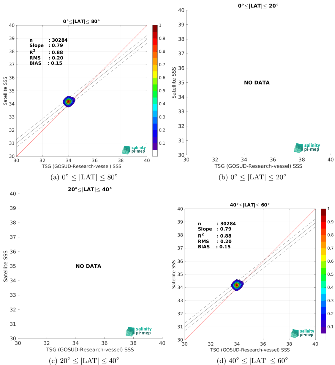
Figure 9: Contour maps of the concentration of Aquarius SSS L3 OR v5 - Monthly - Rain mask (NASA-GSFC) SSS (y-axis) versus TSG (GOSUD-Research-vessel) SSS (x-axis) at match-up pairs for different latitude bands. For each plot, the red line shows x=y . The black thin and dashed lines indicate a linear fit through the data cloud and the \pm 95\% confidence levels, respectively. The number match-up pairs n , the slope and R^2 coefficient of the linear fit, the root mean square (RMS) and the mean bias between satellite and in situ data are indicated for each latitude band in each plots.
