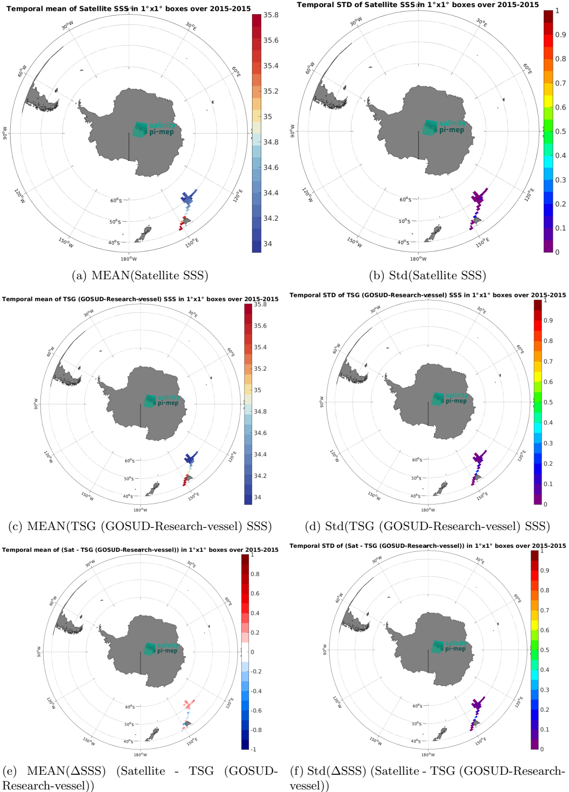
Figure 6: Temporal mean (left) and Std (right) of SSS from Aquarius SSS L3 OR v5 - Monthly - Rain mask (NASA-GSFC) (top), TSG (GOSUD-Research-vessel) (middle), and of \Delta SSS (Satellite - TSG (GOSUD-Research-vessel)). Only 16 up-ch pairs are used to generate these maps.
