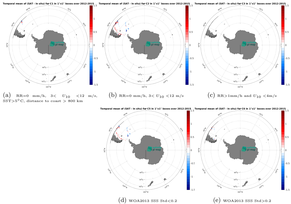
Figure 14: Temporal mean gridded over spatial boxes of size 1^\circ \times 1^\circ of \Delta SSS (Aquarius SSS L3 OR v5 - Monthly - Rain mask (NASA-GSFC) - TSG (CSIC-UTM)) for 5 different subdatasets corresponding to: RR=0 mm/h, 3 < U_{10} < 12 m/s, SST > 5^\circ\text{C} , distance to coast > 800 km (a), RR=0 mm/h, 3 < U_{10} < 12 m/s (b), RR > 1 mm/h and U_{10} < 4 m/s (c), WOA2013 SSS Std < 0.2 (d), WOA2013 SSS Std > 0.2 (e).
