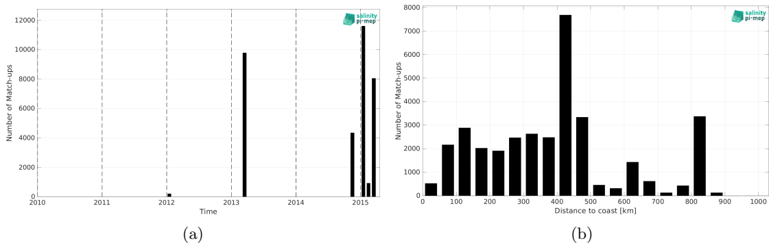
Figure 2: Number of match-ups between TSG (CSIC-UTM) and Aquarius SSS L3 OR v5 - Monthly - Rain mask (NASA-GSFC) SSS as a function of time (a) and as function of the distance to coast (b) over the Roaring Forties and Furious Fifties Pi-MEP region and for the full satellite product period.
