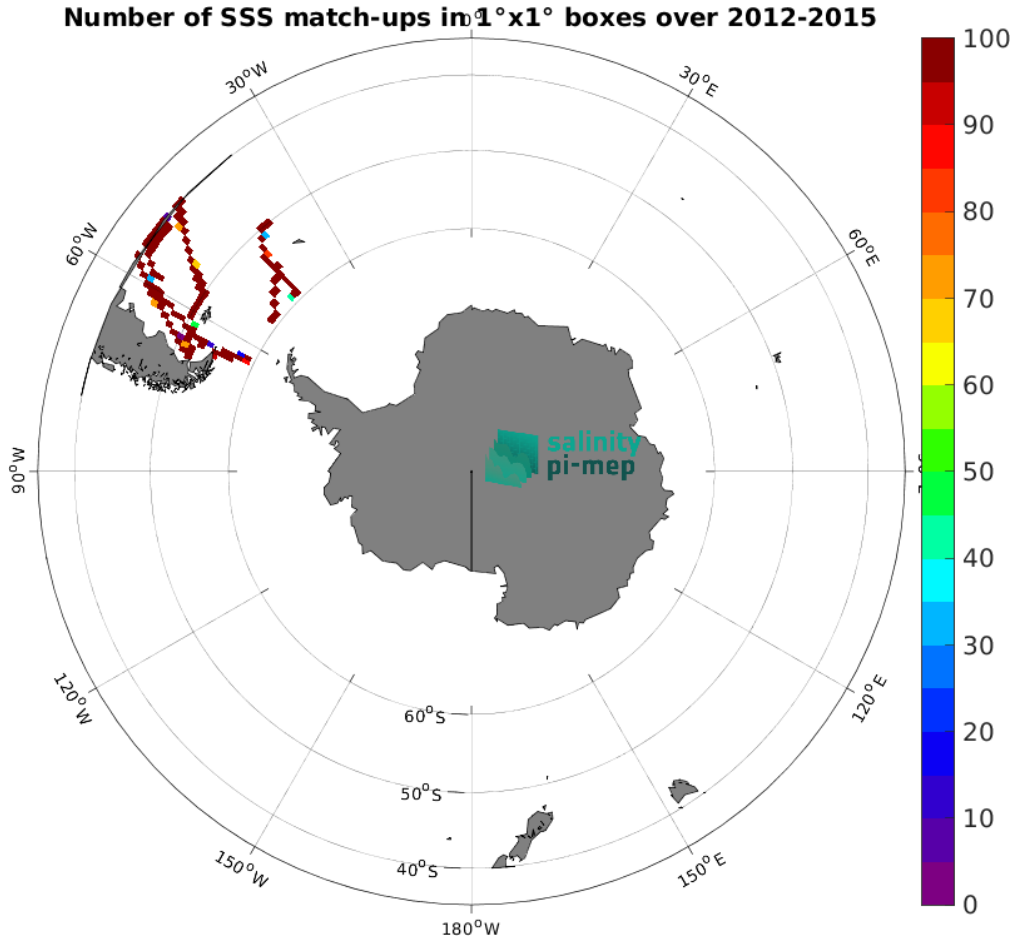
Figure 5: Number of SSS match-ups between TSG (CSIC-UTM) SSS and the Aquarius SSS L3 OR v5 - Monthly - Rain mask (NASA-GSFC) SSS product for the Roaring Forties and Furious Fifties Pi-MEP region over 1^\circ \times 1^\circ boxes and for the full satellite product period.
