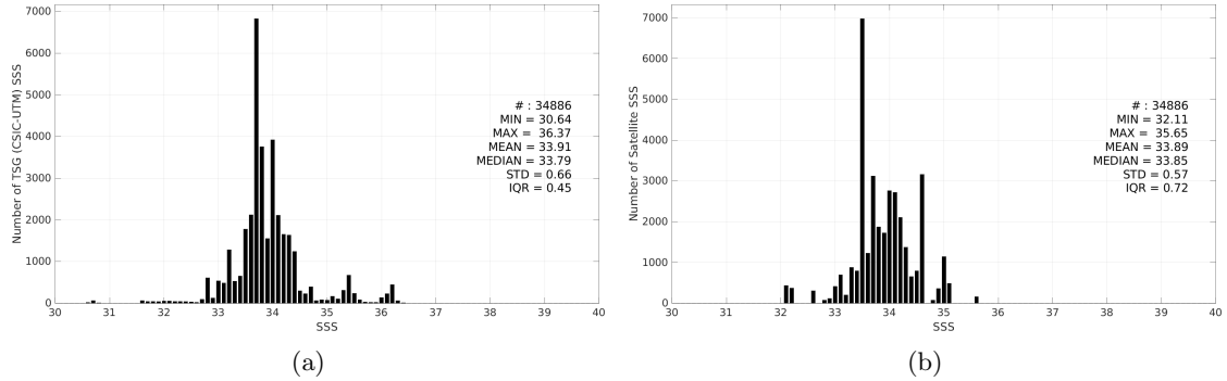
Figure 3: Histograms of SSS from TSG (CSIC-UTM) (a) and Aquarius SSS L3 OR v5 - Monthly - Rain mask (NASA-GSFC) (b) considering all match-up pairs per bins of 0.1 over the Roaring Forties and Furious Fifties Pi-MEP region and for the full satellite product period.
