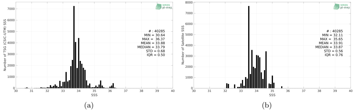
Figure 2: Histograms of SSS from TSG (CSIC-UTM) (a) and Aquarius SSS L3 OR v5 - Monthly - Rain mask (NASA-GSFC) (b) considering all match-up pairs per bins of 0.1 over the Roaring Forties and Furious Fifties Pi-MEP region and for the full satellite product period.
