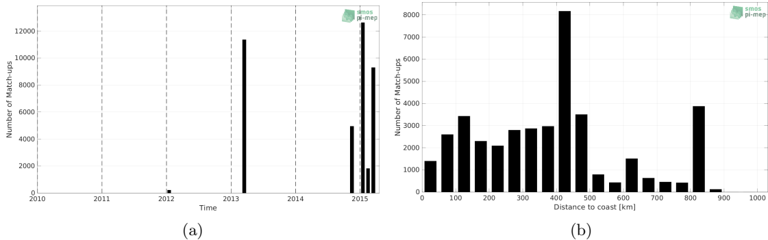
Figure 1: Number of match-ups between TSG (CSIC-UTM) and Aquarius SSS L3 OR v5 - Monthly - Rain mask (NASA-GSFC) SSS as a function of time (a) and as function of the distance to coast (b) over the Roaring Forties and Furious Fifties Pi-MEP region and for the full satellite product period.
