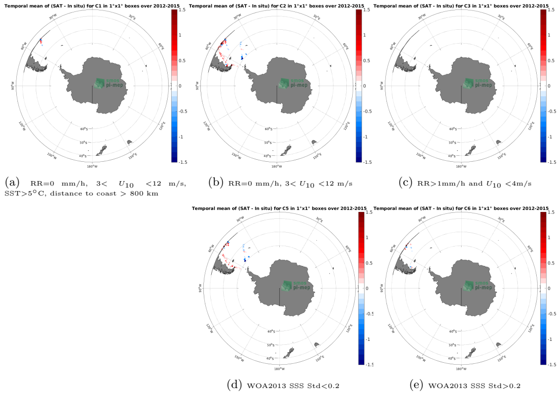
Figure 12: Temporal mean gridded over spatial boxes of size 1^{\circ}\times 1^{\circ} of \Delta\text{SSS} (Aquarius SSS L3 OR v5 - Monthly - Rain mask (NASA-GSFC) - TSG (CSIC-UTM)) for 5 different subdatasets corresponding to:RR=0 mm/h, 3 < U_{10} < 12 m/s, SST >5^{\circ}\text{C} , distance to coast > 800 km (a), RR=0 mm/h, 3 < U_{10} < 12 m/s (b), RR >1 mm/h and U_{10} < 4 m/s (c), WOA2013 SSS Std <0.2 (d), WOA2013 SSS Std >0.2 (e).
