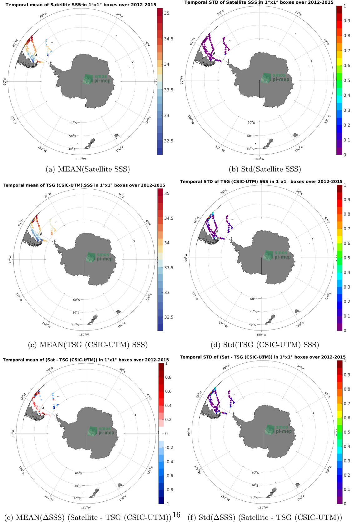
Figure 6: Temporal mean (left) and Std (right) of SSS from Aquarius SSS L3 OR v5 - Monthly - Rain mask (NASA-GSFC) (top), TSG (CSIC-UTM) (middle), and of \Delta SSS (Satellite - TSG (CSIC-UTM)). Only match-up pairs are used to generate these maps.
