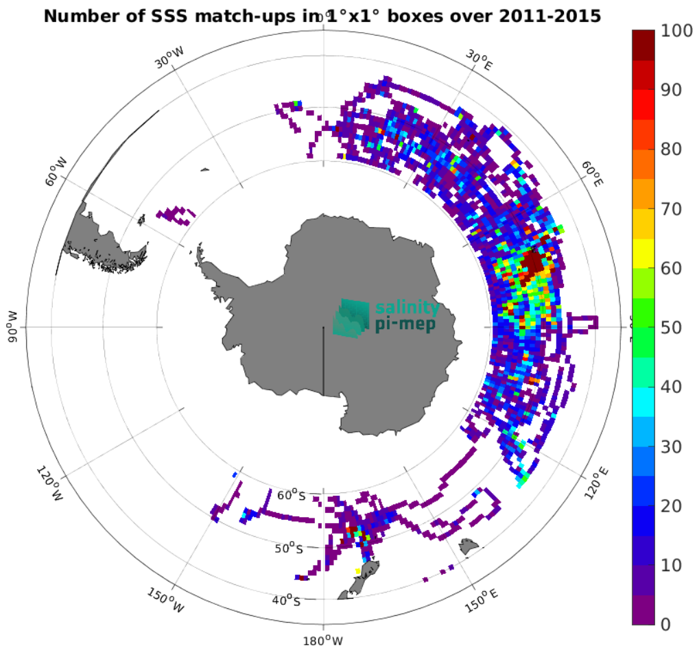
Figure 5: Number of SSS match-ups between Marine mammals SSS and the Aquarius SSS L3 OR v5 - Monthly - Rain mask (NASA-GSFC) SSS product for the Roaring Forties and Furious Fifties Pi-MEP region over 1^\circ \times 1^\circ boxes and for the full satellite product period.
