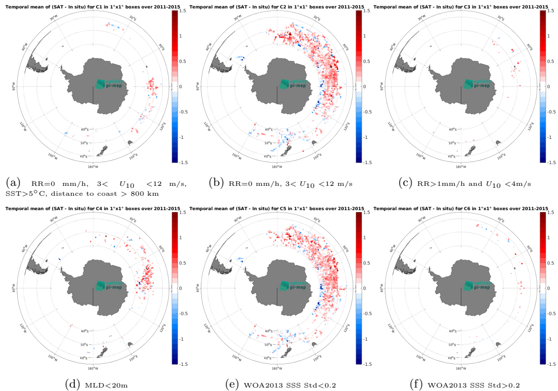
Figure 14: Temporal mean gridded over spatial boxes of size 1^\circ \times 1^\circ of \Delta SSS (Aquarius SSS L3 OR v5 - Monthly - Rain mask (NASA-GSFC) - Marine mammals) for 6 different subdatasets corresponding to:RR=0 mm/h, 3 < U_{10} < 12 m/s, SST>5°C, distance to coast > 800 km (a), RR=0 mm/h, 3 < U_{10} < 12 m/s (b), RR>1mm/h and U_{10} < 4 m/s (c),MLD<20m (d),WOA2013 SSS Std<0.2 (e),WOA2013 SSS Std>0.2 (f).
