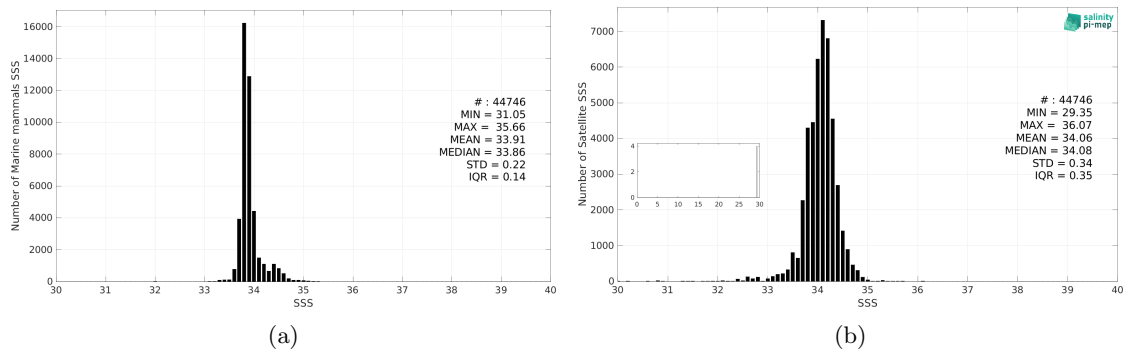
Figure 3: Histograms of SSS from Marine mammals (a) and Aquarius SSS L3 OR v5 - Monthly - Rain mask (NASA-GSFC) (b) considering all match-up pairs per bins of 0.1 over the Roaring Forties and Furious Fifties Pi-MEP region and for the full satellite product period.
