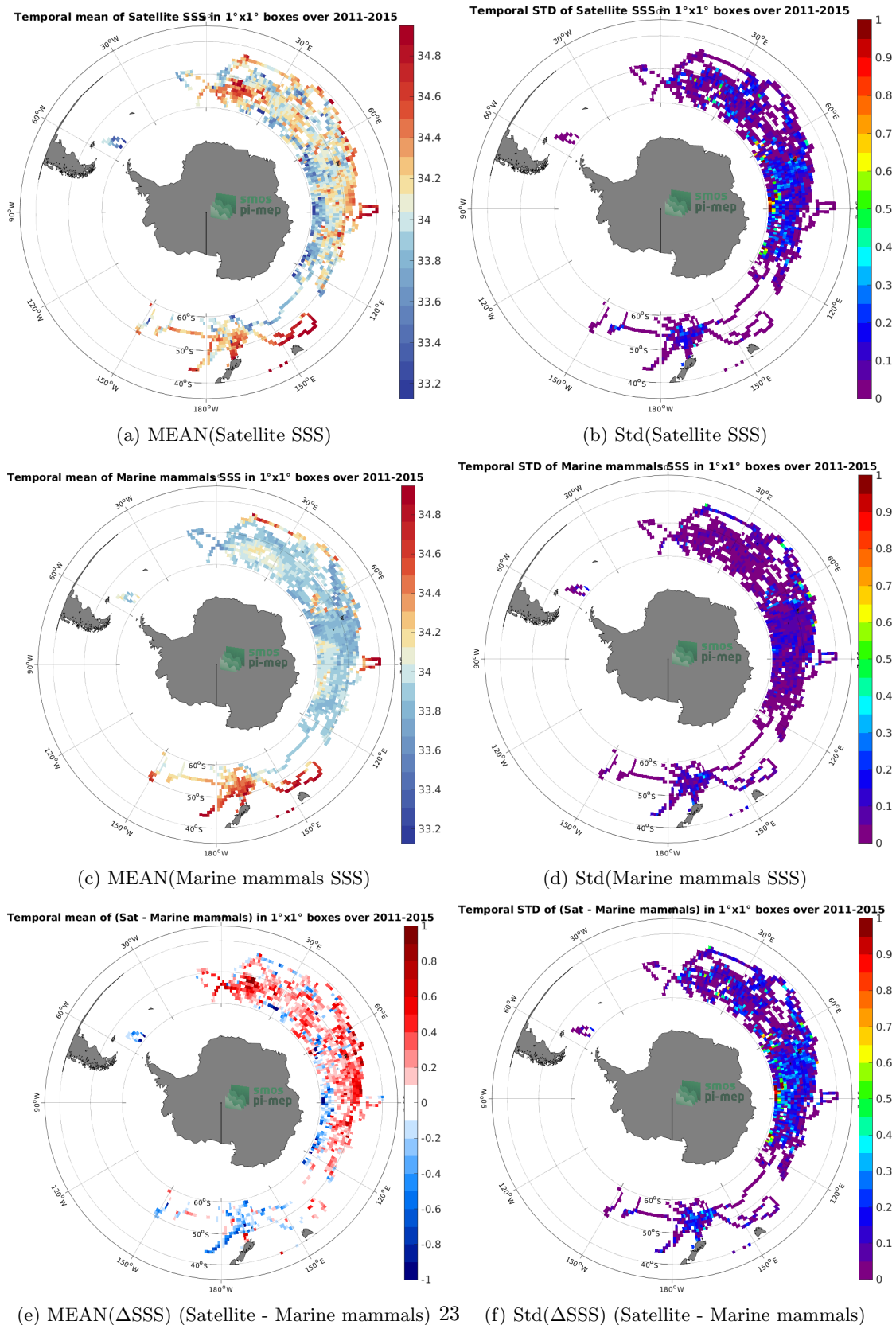
Figure 6: Temporal mean (left) and Std (right) of SSS from Aquarius SSS L3 OR v5 - Monthly - Rain mask (NASA-GSFC) (top), Marine mammals (middle), and of \Delta SSS (Satellite - Marine mammals). Only match-up pairs are used to generate these maps.
