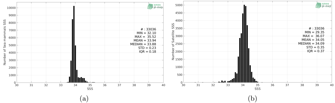
Figure 2: Histograms of SSS from Marine mammals (a) and Aquarius SSS L3 OR v5 - Monthly - Rain mask (NASA-GSFC) (b) considering all match-up pairs per bins of 0.1 over the Roaring Forties and Furious Fifties Pi-MEP region and for the full satellite product period.
