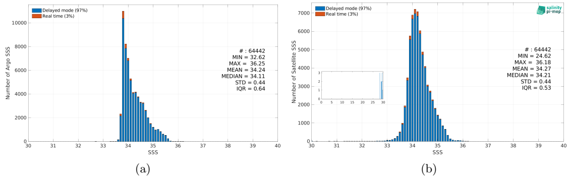
Figure 3: Histograms of SSS from Argo (a) and Aquarius SSS L3 OR v5 - Monthly - Rain mask (NASA-GSFC) (b) considering all match-up pairs per bins of 0.1 over the Roaring Forties and Furious Fifties Pi-MEP region and for the full satellite product period.
