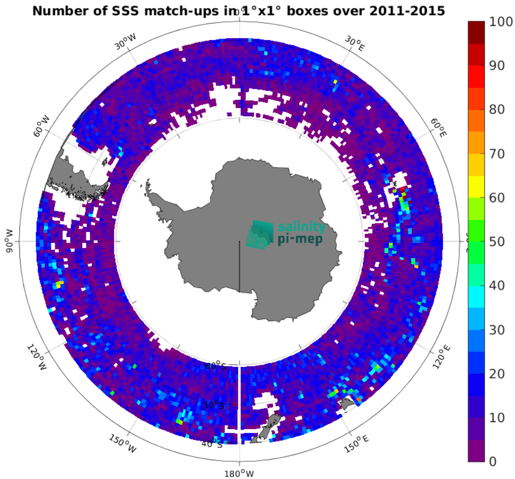
Figure 5: Number of SSS match-ups between Argo SSS and the Aquarius SSS L3 OR v5 - Monthly - Rain mask (NASA-GSFC) SSS product for the Roaring Forties and Furious Fifties Pi-MEP region over 1^\circ \times 1^\circ boxes and for the full satellite product period.
