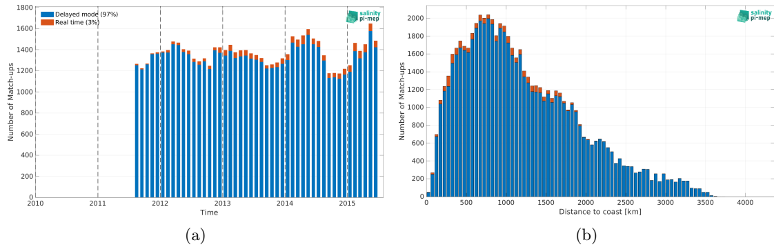
Figure 2: Number of match-ups between Argo and Aquarius SSS L3 OR v5 - Monthly - Rain mask (NASA-GSFC) SSS as a function of time (a) and as function of the distance to coast (b) over the Roaring Forties and Furious Fifties Pi-MEP region and for the full satellite product period.
