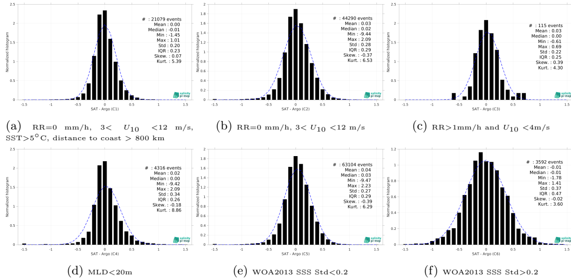
Figure 13: Normalized histogram of \Delta\text{SSS} (Aquarius SSS L3 OR v5 - Monthly - Rain mask (NASA-GSFC) - Argo) for 6 different subdatasets corresponding to: RR=0 mm/h, 3 < U_{10} < 12 m/s, SST>5°C, distance to coast > 800 km (a), RR=0 mm/h, 3 < U_{10} < 12 m/s (b), RR>1mm/h and U_{10} < 4 m/s (c), MLD<20m (d), WOA2013 SSS Std<0.2 (e), WOA2013 SSS Std>0.2 (f).
