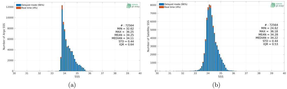
Figure 2: Histograms of SSS from Argo (a) and Aquarius SSS L3 OR v5 - Monthly - Rain mask (NASA-GSFC) (b) considering all match-up pairs per bins of 0.1 over the Roaring Forties and Furious Fifties Pi-MEP region and for the full satellite product period.
