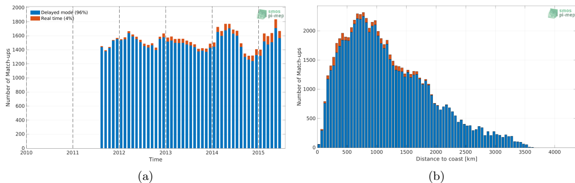
Figure 1: Number of match-ups between Argo and Aquarius SSS L3 OR v5 - Monthly - Rain mask (NASA-GSFC) SSS as a function of time (a) and as function of the distance to coast (b) over the Roaring Forties and Furious Fifties Pi-MEP region and for the full satellite product period.
