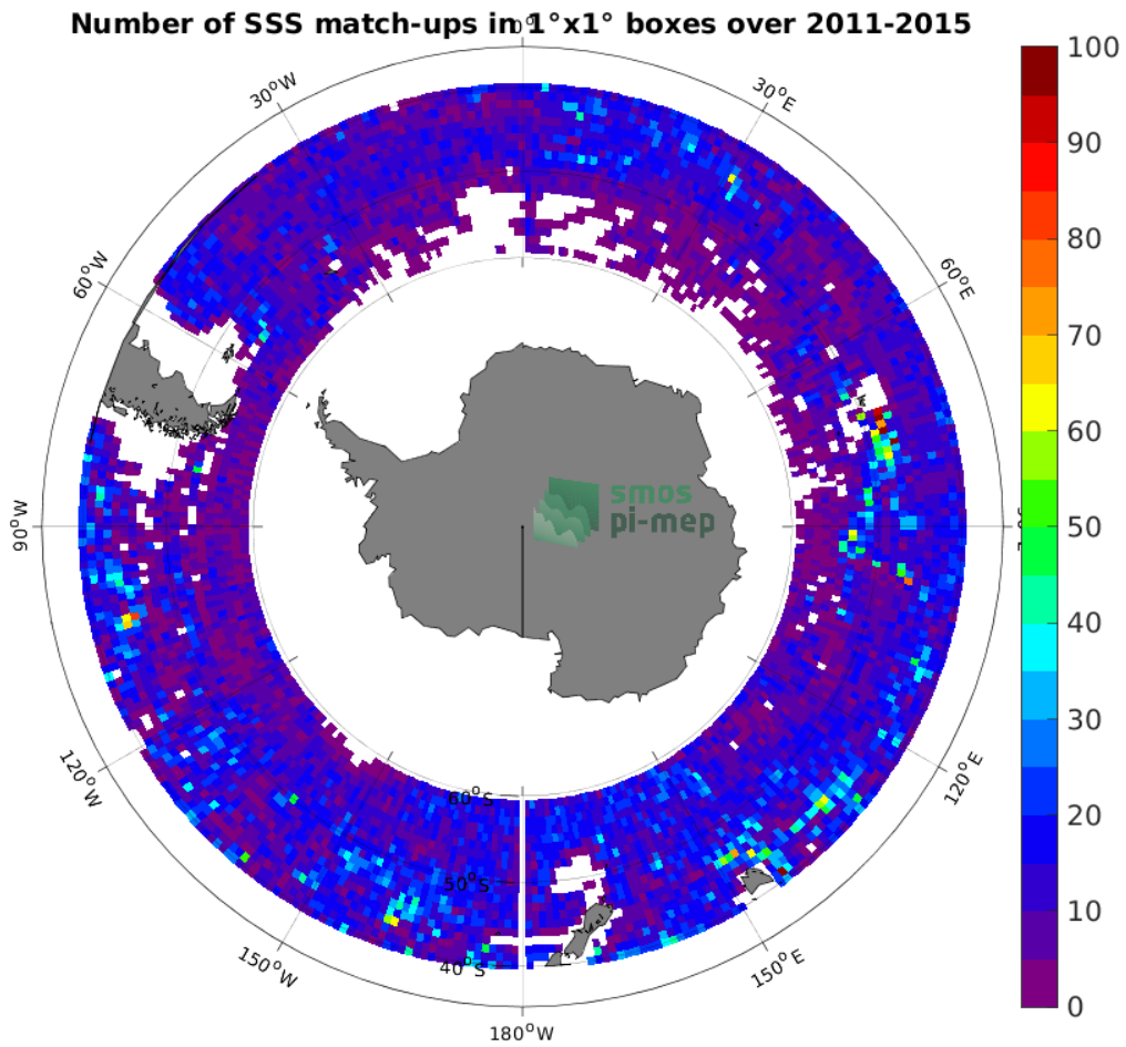
Figure 4: Number of SSS match-ups between Argo SSS and the Aquarius SSS L3 OR v5 - Monthly - Rain mask (NASA-GSFC) SSS product for the Roaring Forties and Furious Fifties Pi-MEP region over 1^\circ \times 1^\circ boxes and for the full satellite product period.
