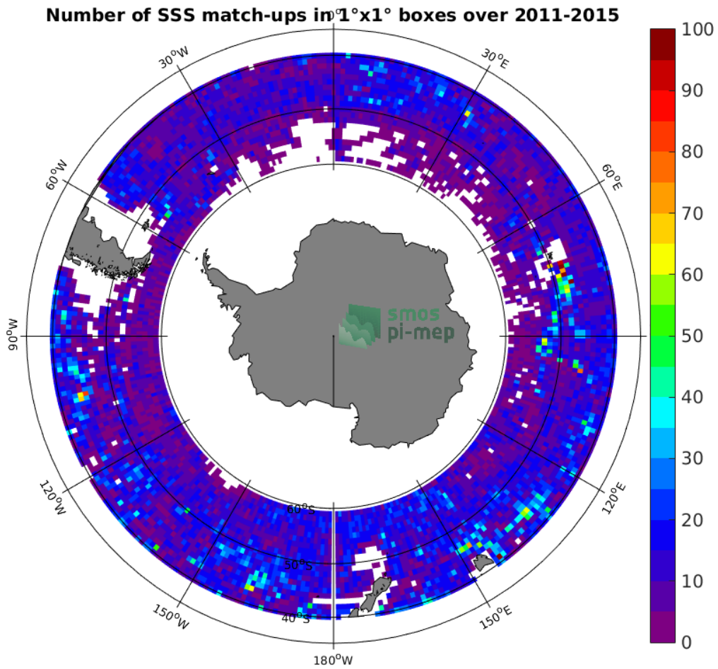
Figure 4: Number of SSS match-ups between Argo SSS and the Aquarius-L3-OR-V5-MONTHLY-RAIN-MASK-1DEG SSS product for the Roaring Forties and Furious Fifties Pi-MEP region over 1°x1° boxes and for the full satellite product period.
