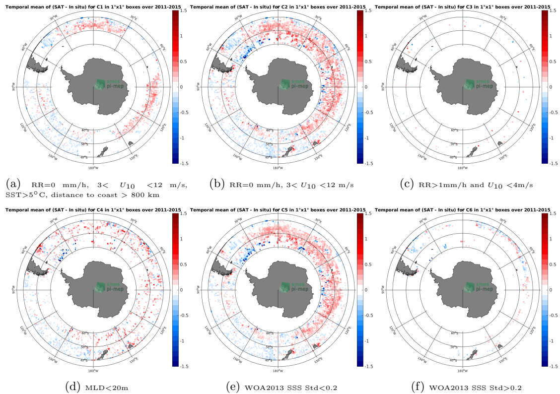
Figure 12: Temporal mean gridded over spatial boxes of size 1^{\circ}\times 1^{\circ} of \Delta\text{SSS} (Aquarius-L3-OR-V5-MONTHLY-RAIN-MASK-1DEG - Argo) for 6 different subdatasets corresponding to: RR=0 mm/h, 3 < U_{10} < 12 m/s, SST > 5^{\circ}\text{C} , distance to coast > 800 km (a), RR=0 mm/h, 3 < U_{10} < 12 m/s (b), RR > 1\text{mm/h} and U_{10} < 4\text{m/s} (c), MLD < 20\text{m} (d), WOA2013 SSS Std < 0.2 (e), WOA2013 SSS Std > 0.2 (f).
