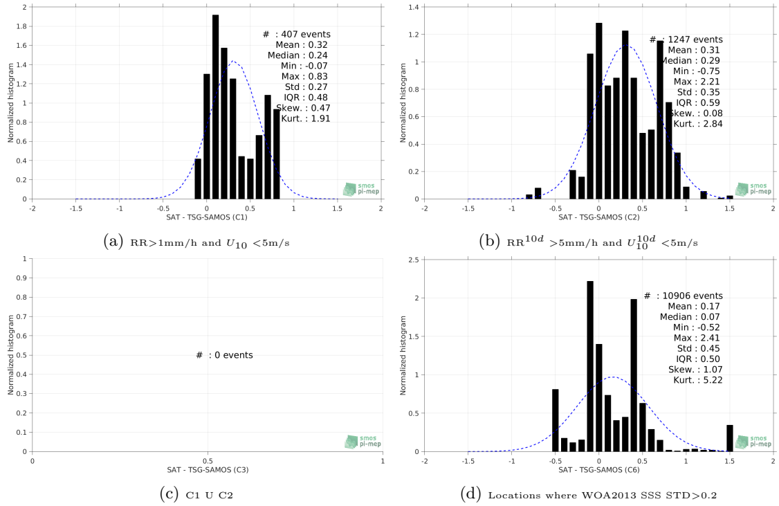
Figure 13: Normalized histogram of \Delta\text{SSS} (Aquarius-L3-JPL-V5-7DAY-RUNNING - TSG-SAMOS) for 6 different subdatasets corresponding to: RR > 1\text{mm/h} and U_{10} < 5\text{m/s} (a), RR^{10d} > 5\text{mm/h} and U_{10}^{10d} < 5\text{m/s} (b), C1 \cup C2 (c), Locations where WOA2013 SSS STD > 0.2 (d).
