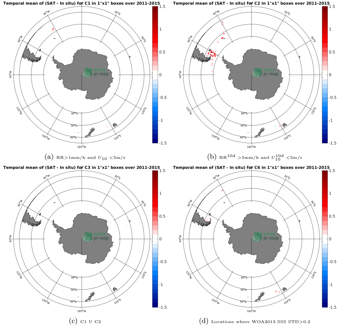
Figure 12: Temporal mean gridded over spatial boxes of size 1^\circ \times 1^\circ of \Delta SSS (Aquarius-L3-JPL-V5-7DAY-RUNNING - TSG-SAMOS) for 4 different subdatasets corresponding to:RR > 1\text{mm/h} and U_{10} < 5\text{m/s} (a), RR^{10d} > 5\text{mm/h} and U_{10}^{10d} < 5\text{m/s} (b), C1 U C2 (c), Locations where WOA2013 SSS STD > 0.2 (d).
