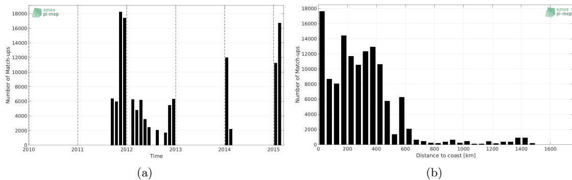
Figure 1: Number of match-ups between TSG-SAMOS and Aquarius-L3-JPL-V5-7DAY-RUNNING SSS as a function of time (a) and as function of the distance to coast (b) over the Roaring Forties and Furious Fifties Pi-MEP region and for the full satellite product period.
