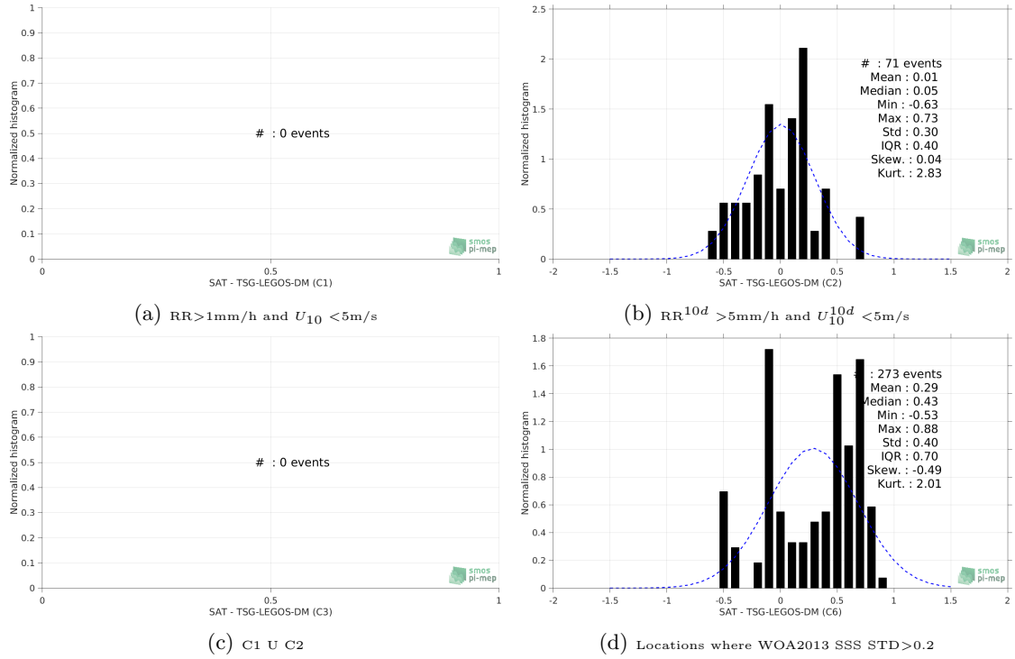
Figure 13: Normalized histogram of \Delta\text{SSS} (Aquarius-L3-JPL-V5-7DAY-RUNNING - TSG-LEGOS-DM) for 6 different subdatasets corresponding to: RR > 1\text{mm/h} and U_{10} < 5\text{m/s} (a), RR^{10d} > 5\text{mm/h} and U_{10}^{10d} < 5\text{m/s} (b), C1 \cup C2 (c), Locations where WOA2013 SSS STD > 0.2 (d).
