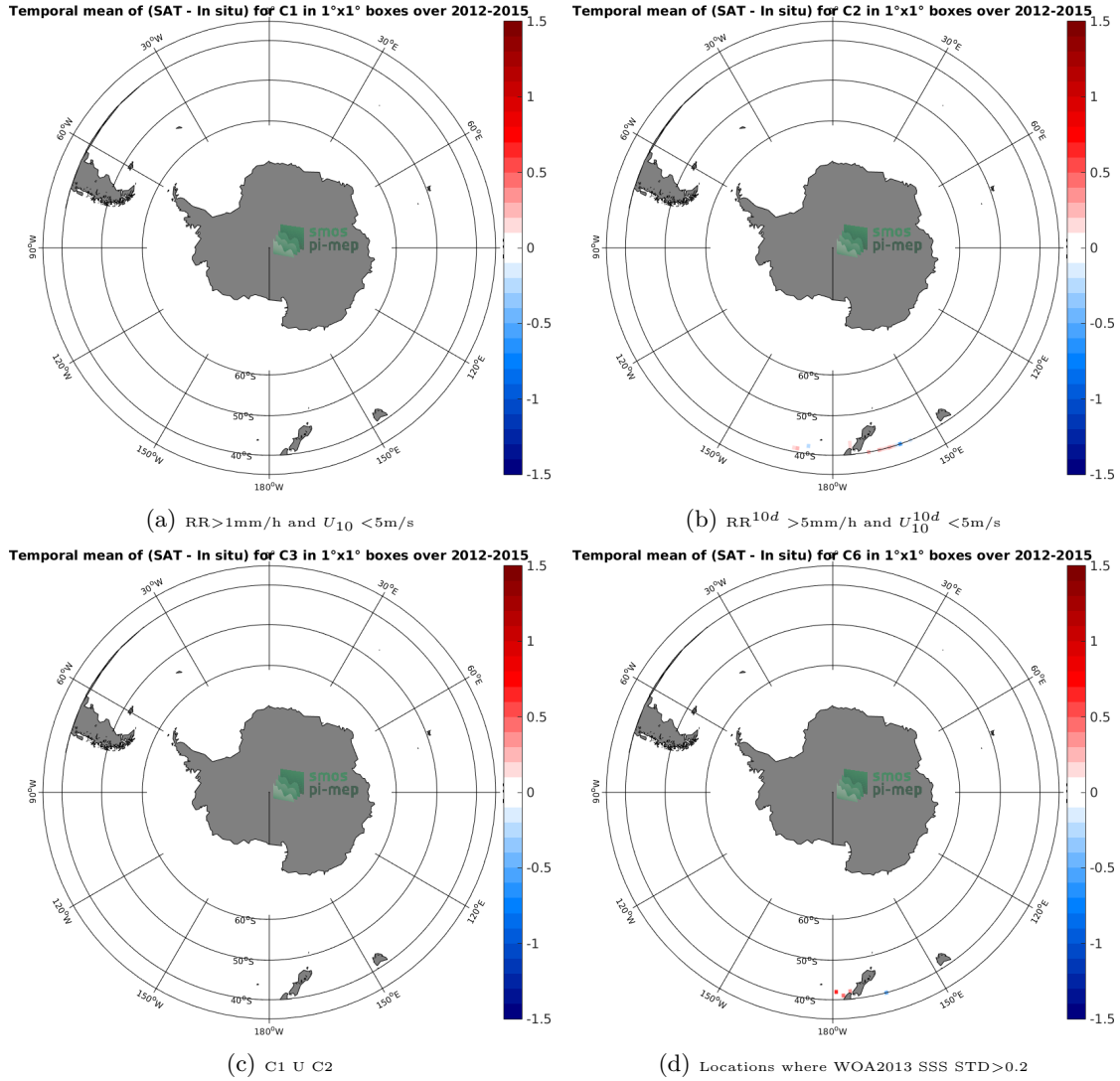
Figure 12: Temporal mean gridded over spatial boxes of size 1^\circ \times 1^\circ of \Delta SSS (Aquarius-L3-JPL-V5-7DAY-RUNNING - TSG-LEGOS-DM) for 4 different subdatasets corresponding to: RR > 1mm/h and U_{10} < 5\text{m/s} (a), RR^{10d} > 5\text{mm/h} and U_{10}^{10d} < 5\text{m/s} (b), C1 U C2 (c), Locations where WOA2013 SSS STD > 0.2 (d).
