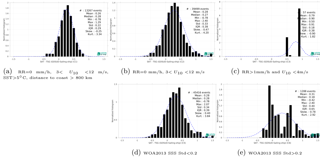
Figure 15: Normalized histogram of \Delta SSS (Aquarius SSS L3 CAP v5 - 7-Day running (JPL) - TSG (GOSUD-Sailing-ship)) for 5 different subdatasets corresponding to: RR=0 mm/h, 3 < U_{10} < 12 m/s, SST>5°C, distance to coast > 800 km (a), RR=0 mm/h, 3 < U_{10} < 12 m/s (b), RR>1mm/h and U_{10} < 4 m/s (c), WOA2013 SSS Std<0.2 (d), WOA2013 SSS Std>0.2 (e).
