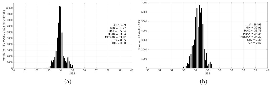
Figure 3: Histograms of SSS from TSG (GOSUD-Sailing-ship) (a) and Aquarius SSS L3 CAP v5 - 7-Day running (JPL) (b) considering all match-up pairs per bins of 0.1 over the Roaring Forties and Furious Fifties Pi-MEP region and for the full satellite product period.
