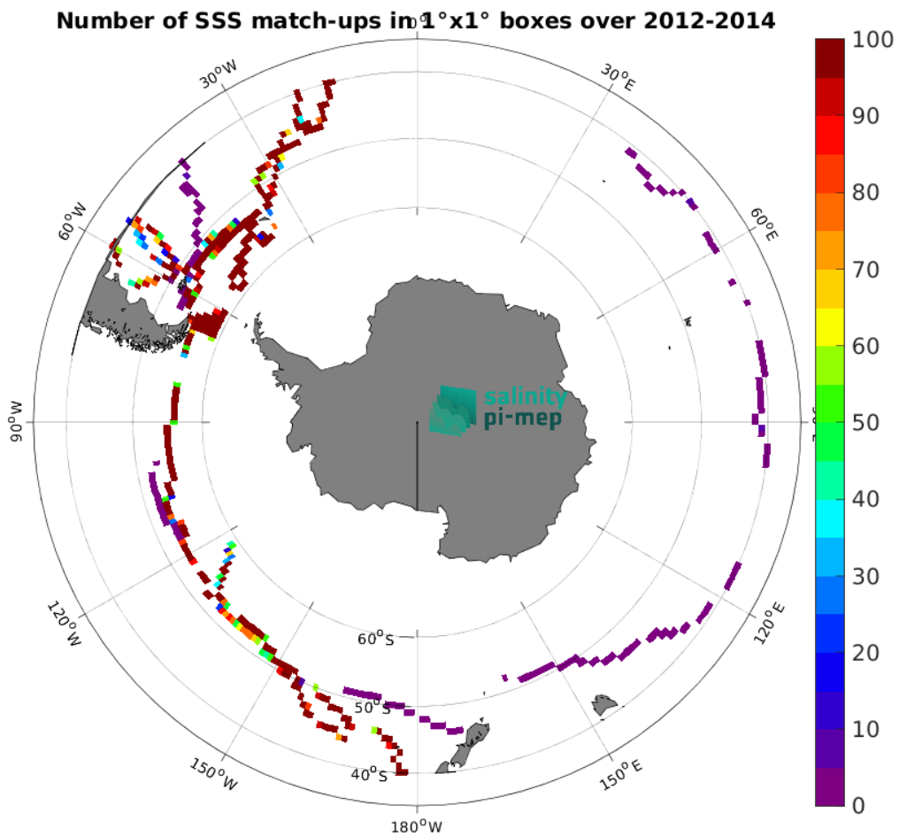
Figure 5: Number of SSS match-ups between TSG (GOSUD-Sailing-ship) SSS and the Aquarius SSS L3 CAP v5 - 7-Day running (JPL) SSS product for the Roaring Forties and Furious Fifties Pi-MEP region over 1^\circ \times 1^\circ boxes and for the full satellite product period.
