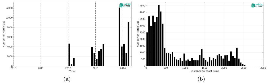
Figure 2: Number of match-ups between TSG (GOSUD-Sailing-ship) and Aquarius SSS L3 CAP v5 - 7-Day running (JPL) SSS as a function of time (a) and as function of the distance to coast (b) over the Roaring Forties and Furious Fifties Pi-MEP region and for the full satellite product period.
