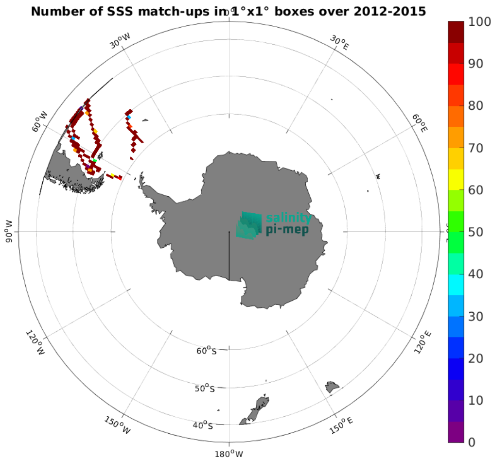
Figure 5: Number of SSS match-ups between TSG (CSIC-UTM) SSS and the Aquarius SSS L3 CAP v5 - 7-Day running (JPL) SSS product for the Roaring Forties and Furious Fifties Pi-MEP region over 1^{\circ} \times 1^{\circ} boxes and for the full satellite product period.
