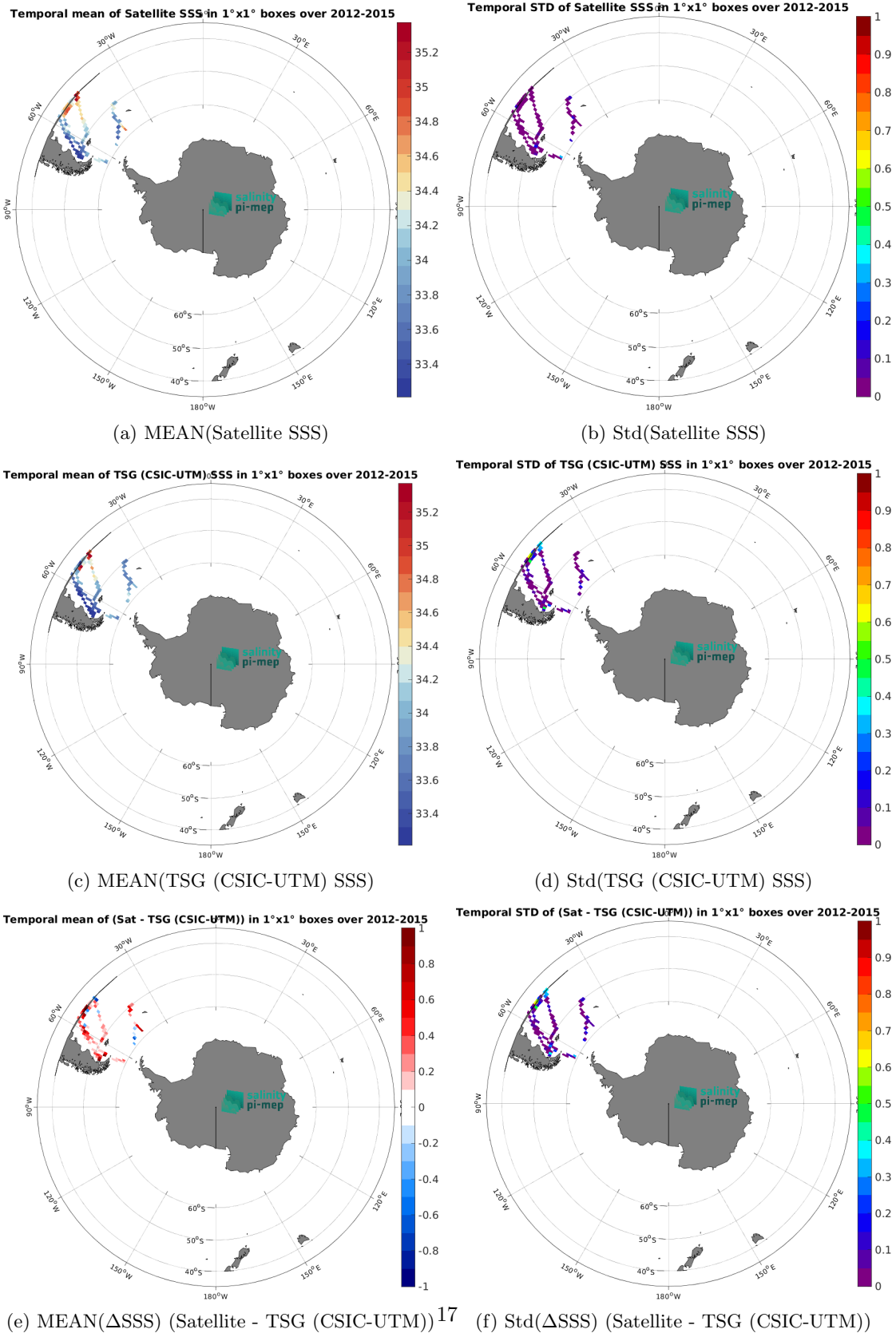
Figure 7: Temporal mean (left) and Std (right) of SSS from Aquarius SSS L3 CAP v5 - 7-Day running (JPL) (top), TSG (CSIC-UTM) (middle), and of \Delta SSS (Satellite - TSG (CSIC-UTM)). Only match-up pairs are used to generate these maps.
