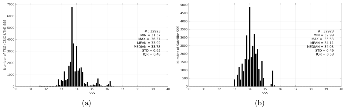
Figure 3: Histograms of SSS from TSG (CSIC-UTM) (a) and Aquarius SSS L3 CAP v5 - 7-Day running (JPL) (b) considering all match-up pairs per bins of 0.1 over the Roaring Forties and Furious Fifties Pi-MEP region and for the full satellite product period.
