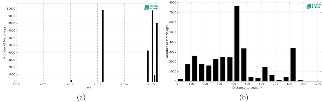
Figure 2: Number of match-ups between TSG (CSIC-UTM) and Aquarius SSS L3 CAP v5 - 7-Day running (JPL) SSS as a function of time (a) and as function of the distance to coast (b) over the Roaring Forties and Furious Fifties Pi-MEP region and for the full satellite product period.
