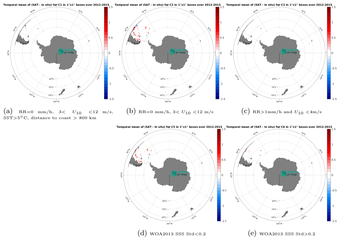
Figure 14: Temporal mean gridded over spatial boxes of size 1^\circ \times 1^\circ of \Delta SSS (Aquarius SSS L3 CAP v5 - 7-Day running (JPL) - TSG (CSIC-UTM)) for 5 different subdatasets corresponding to: RR=0 mm/h, 3 < U_{10} < 12 m/s, SST > 5^\circ\text{C} , distance to coast > 800 km (a), RR=0 mm/h, 3 < U_{10} < 12 m/s (b), RR > 1 mm/h and U_{10} < 4 m/s (c), WOA2013 SSS Std < 0.2 (d), WOA2013 SSS Std > 0.2 (e).
