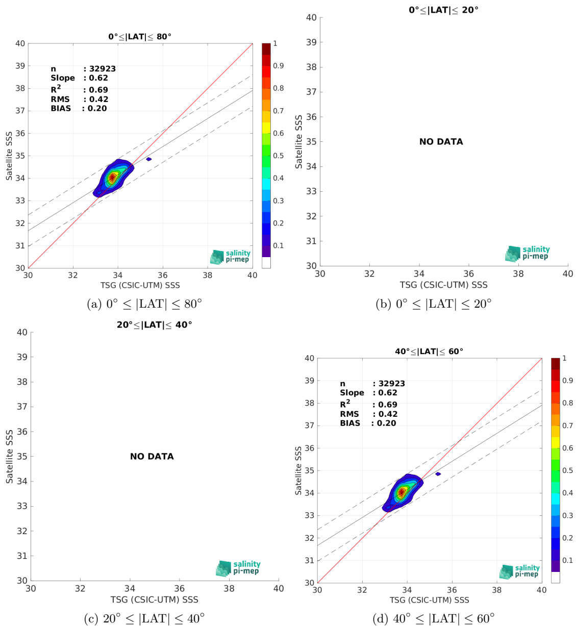
Figure 10: Contour maps of the concentration of Aquarius SSS L3 CAP v5 - 7-Day running (JPL) SSS (y-axis) versus TSG (CSIC-UTM) SSS (x-axis) at match-up pairs for different latitude bands. For each plot, the red line shows x=y . The black thin and dashed lines indicate a linear fit through the data cloud and the \pm 95\% confidence levels, respectively. The number match-up pairs n , the slope and R^2 coefficient of the linear fit, the root mean square (RMS) and the mean bias between satellite and in situ data are indicated for each latitude band in each plot.
