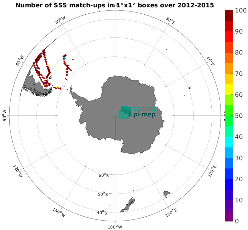
Figure 5: Number of SSS match-ups between TSG (CSIC-UTM) SSS and the Aquarius SSS L3 CAP v5 - 7-Day running (JPL) SSS product for the Roaring Forties and Furious Fifties Pi-MEP region over 1^\circ \times 1^\circ boxes and for the full satellite product period.
