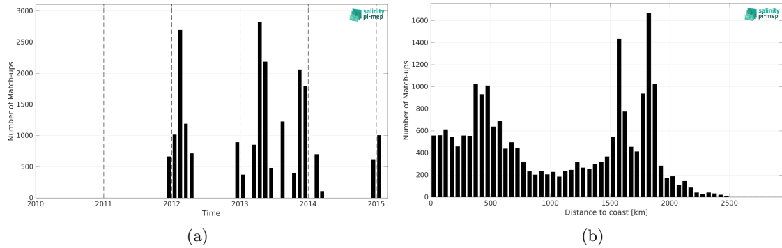
Figure 2: Number of match-ups between TSG (Polarstern) and Aquarius SSS L3 CAP v5 - Monthly (JPL) SSS as a function of time (a) and as function of the distance to coast (b) over the Roaring Forties and Furious Fifties Pi-MEP region and for the full satellite product period.
