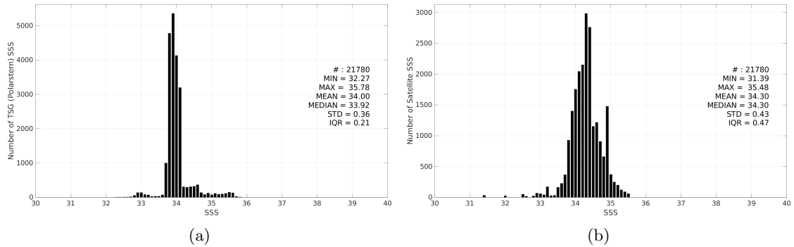
Figure 3: Histograms of SSS from TSG (Polarstern) (a) and Aquarius SSS L3 CAP v5 - Monthly (JPL) (b) considering all match-up pairs per bins of 0.1 over the Roaring Forties and Furious Fifties Pi-MEP region and for the full satellite product period.
