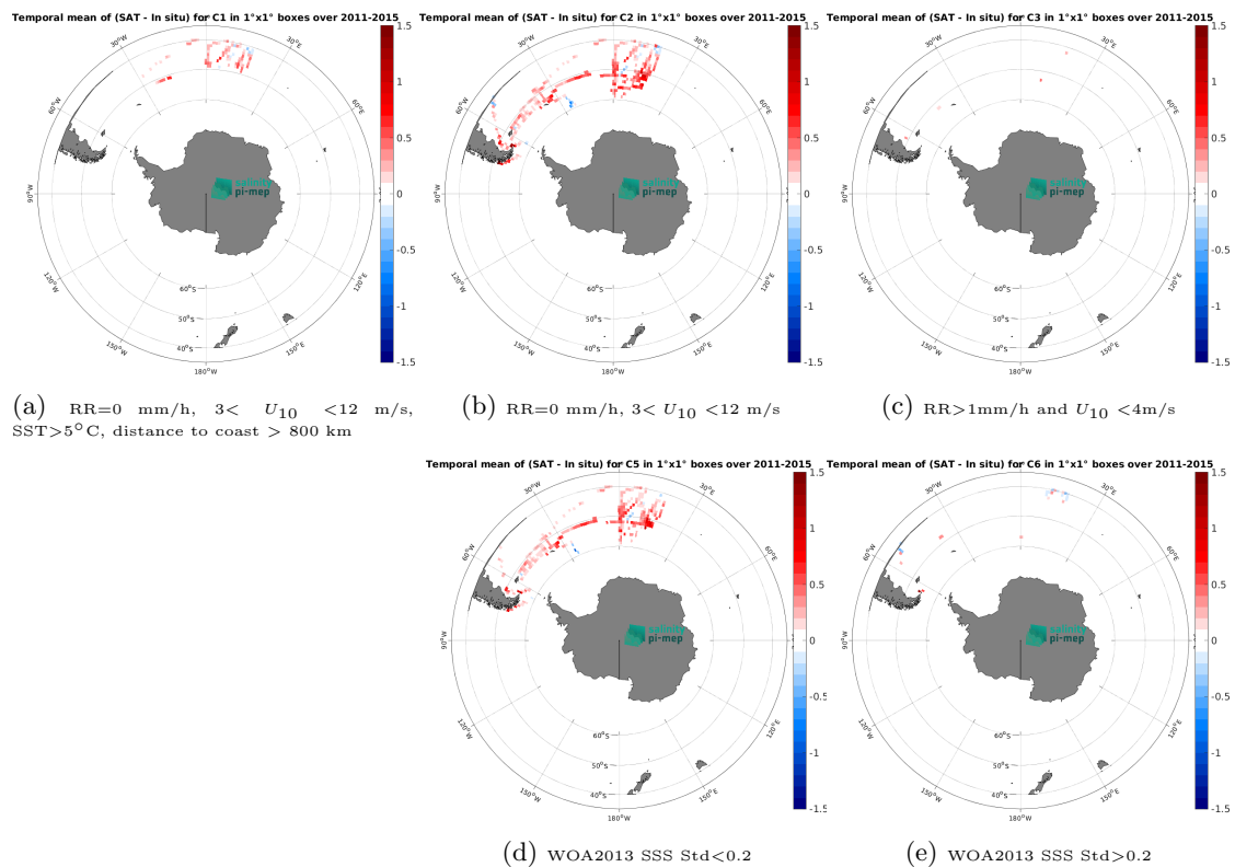
Figure 14: Temporal mean gridded over spatial boxes of size 1^\circ \times 1^\circ of \Delta SSS (Aquarius SSS L3 CAP v5 - Monthly (JPL) - TSG (Polarstern)) for 5 different subdatasets corresponding to: RR=0 mm/h, 3 < U_{10} < 12 m/s, SST > 5^\circ\text{C} , distance to coast > 800 km (a), RR=0 mm/h, 3 < U_{10} < 12 m/s (b), RR > 1 mm/h and U_{10} < 4 m/s (c), WOA2013 SSS Std < 0.2 (d), WOA2013 SSS Std > 0.2 (e).
