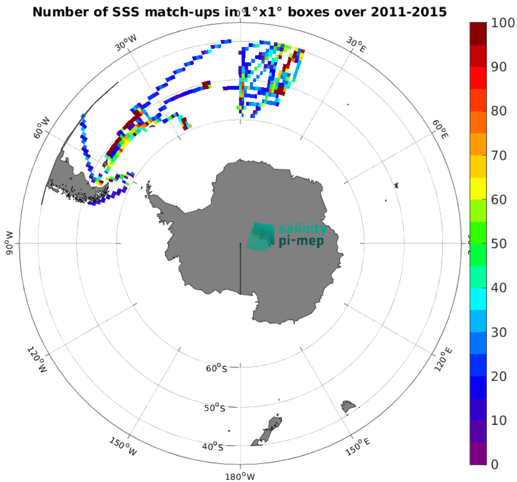
Figure 5: Number of SSS match-ups between TSG (Polarstern) SSS and the Aquarius SSS L3 CAP v5 - Monthly (JPL) SSS product for the Roaring Forties and Furious Fifties Pi-MEP region over 1^\circ \times 1^\circ boxes and for the full satellite product period.
