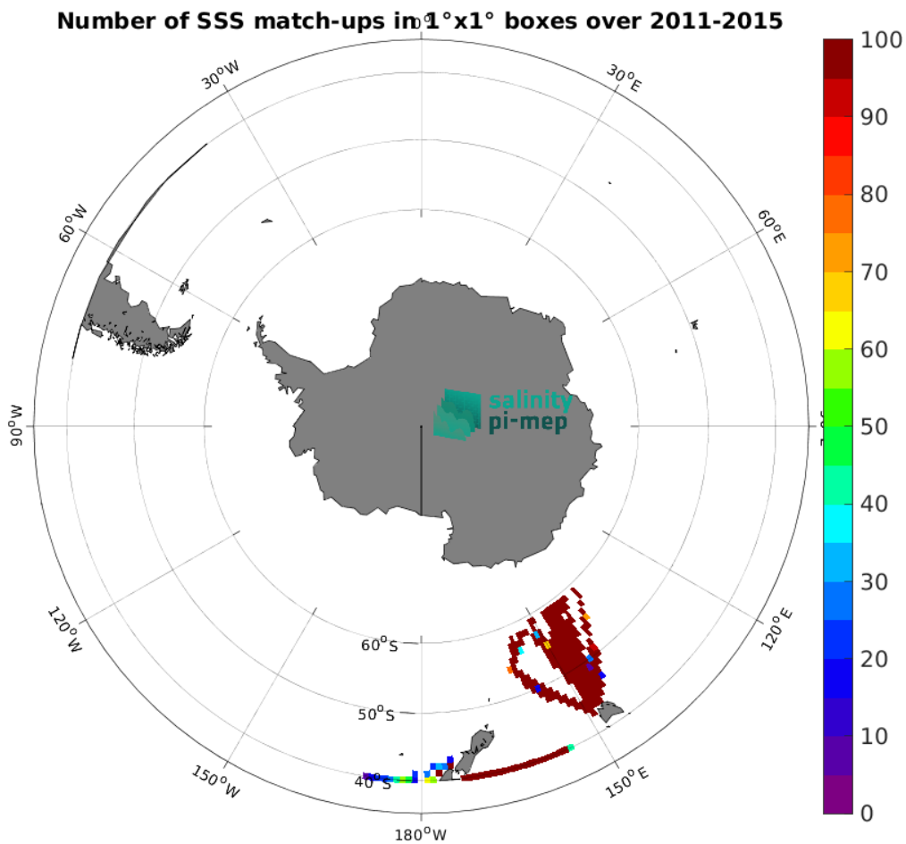
Figure 5: Number of SSS match-ups between TSG (LEGOS-DM) SSS and the Aquarius SSS L3 CAP v5 - Monthly (JPL) SSS product for the Roaring Forties and Furious Fifties Pi-MEP region over 1^\circ \times 1^\circ boxes and for the full satellite product period.
