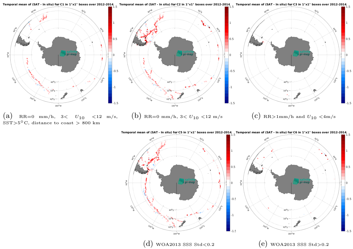
Figure 12: Temporal mean gridded over spatial boxes of size 1^\circ \times 1^\circ of \Delta SSS (Aquarius SSS L3 CAP v5 - Monthly (JPL) - TSG (GOSUD-Sailing-ship)) for 5 different subdatasets corresponding to: RR=0 mm/h, 3 < U_{10} < 12 m/s, SST>5°C, distance to coast > 800 km (a), RR=0 mm/h, 3 < U_{10} < 12 m/s (b), RR>1mm/h and U_{10} < 4 m/s (c), WOA2013 SSS Std<0.2 (d), WOA2013 SSS Std>0.2 (e).
