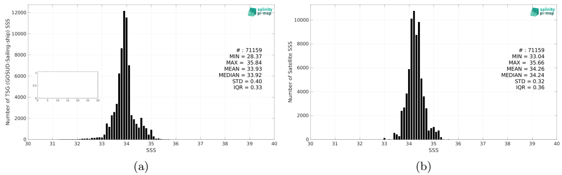
Figure 2: Histograms of SSS from TSG (GOSUD-Sailing-ship) (a) and Aquarius SSS L3 CAP v5 - Monthly (JPL) (b) considering all match-up pairs per bins of 0.1 over the Roaring Forties and Furious Fifties Pi-MEP region and for the full satellite product period.
