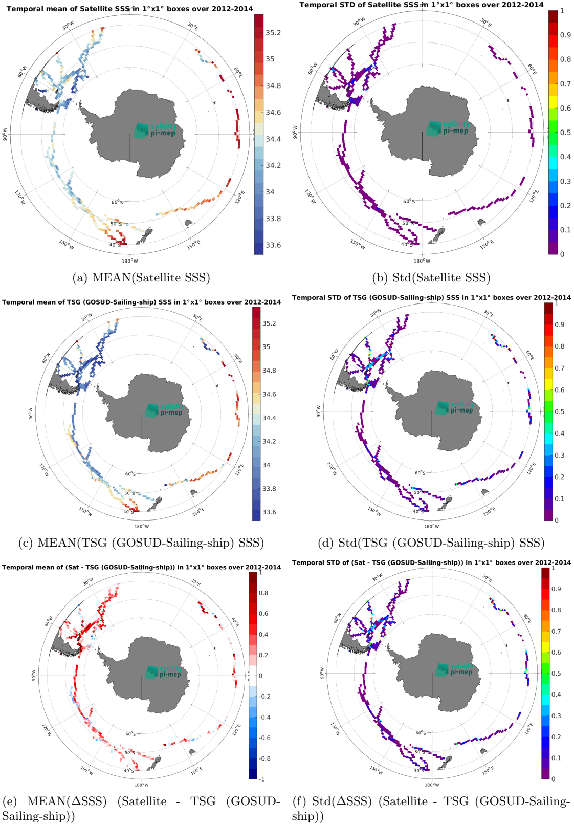
Figure 6: Temporal mean (left) and Std (right) of SSS from Aquarius SSS L3 CAP v5 - Monthly (JPL) (top), TSG (GOSUD-Sailing-ship) (middle), and of \Delta SSS (Satellite - TSG (GOSUD-Sailing-ship)). Only match-up pairs are used to generate these maps.
