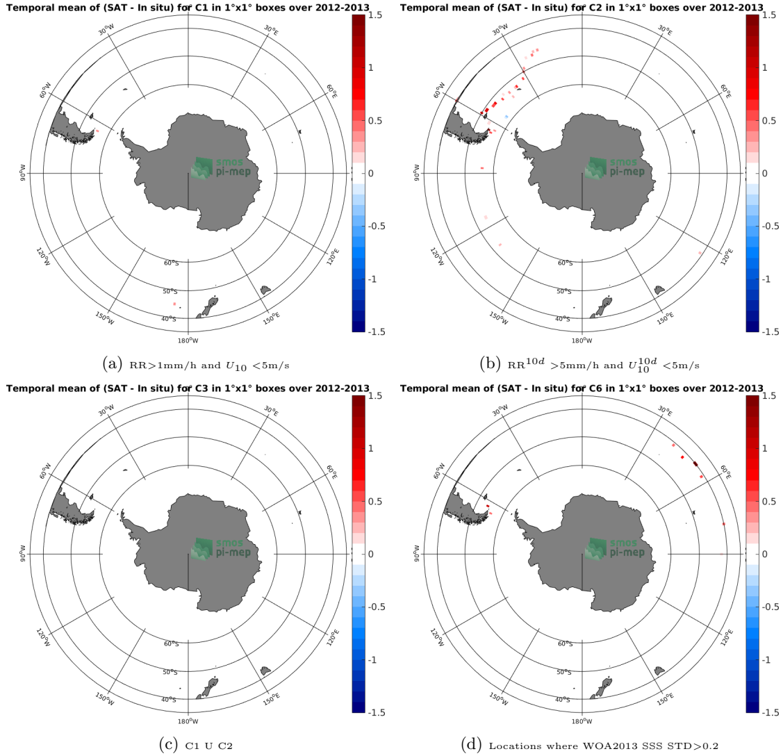
Figure 12: Temporal mean gridded over spatial boxes of size 1^\circ \times 1^\circ of \Delta SSS (Aquarius-L3-JPL-V5-MONTHLY - TSG-GOSUD-Sailing-ship) for 4 different subdatasets corresponding to: RR > 1\text{mm/h} and U_{10} < 5\text{m/s} (a), RR^{10d} > 5\text{mm/h} and U_{10}^{10d} < 5\text{m/s} (b), C1 U C2 (c), Locations where WOA2013 SSS STD > 0.2 (d).
