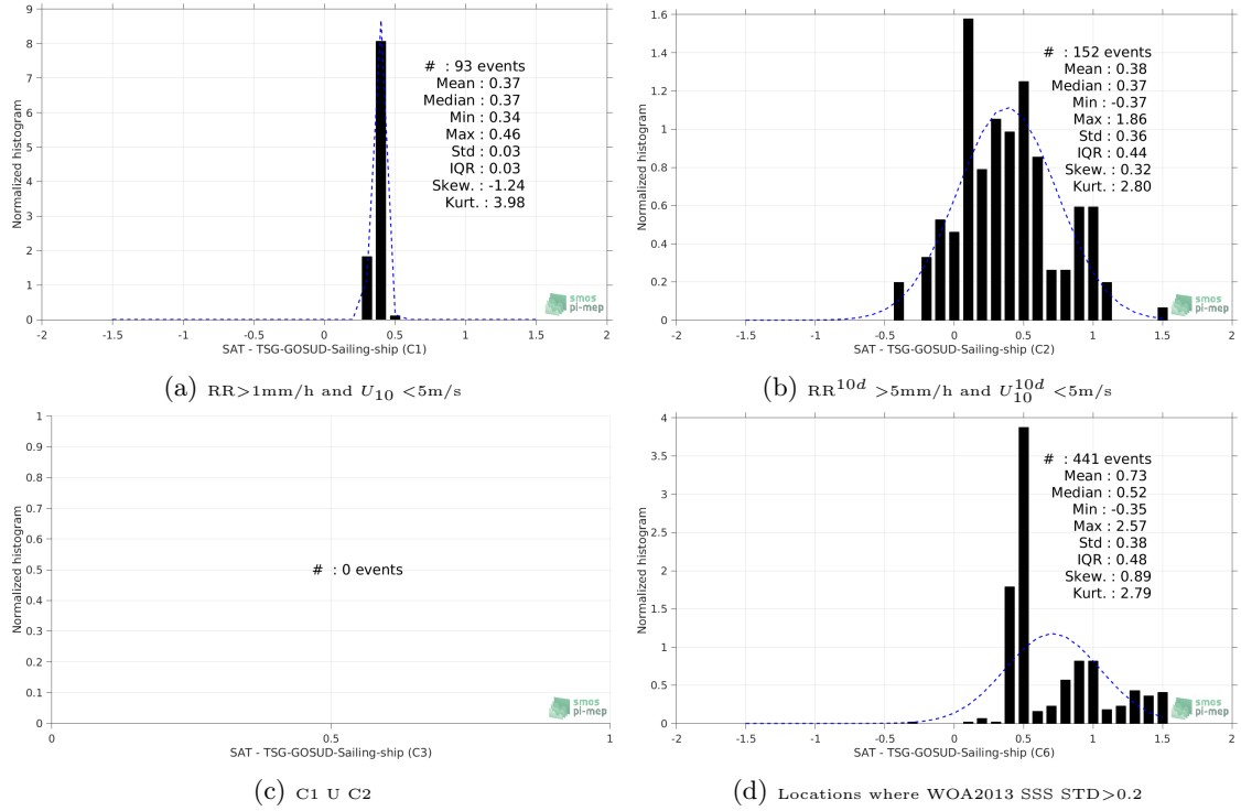
Figure 13: Normalized histogram of \Delta\text{SSS} (Aquarius-L3-JPL-V5-MONTHLY - TSG-GOSUD-Sailing-ship) for 6 different subdatasets corresponding to: RR > 1mm/h and U_{10} < 5\text{m/s} (a), RR^{10d} > 5\text{mm/h} and U_{10}^{10d} < 5\text{m/s} (b), C1 U C2 (c), Locations where WOA2013 SSS STD > 0.2 (d).
