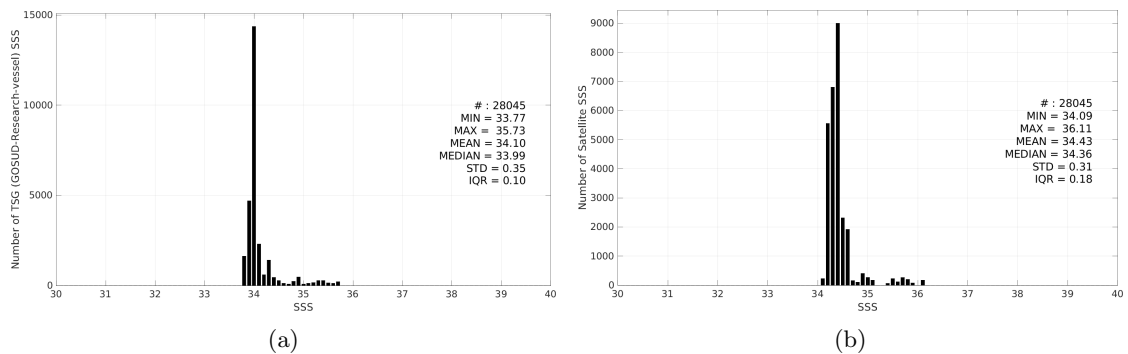
Figure 3: Histograms of SSS from TSG (GOSUD-Research-vessel) (a) and Aquarius SSS L3 CAP v5 - Monthly (JPL) (b) considering all match-up pairs per bins of 0.1 over the Roaring Forties and Furious Fifties Pi-MEP region and for the full satellite product period.
