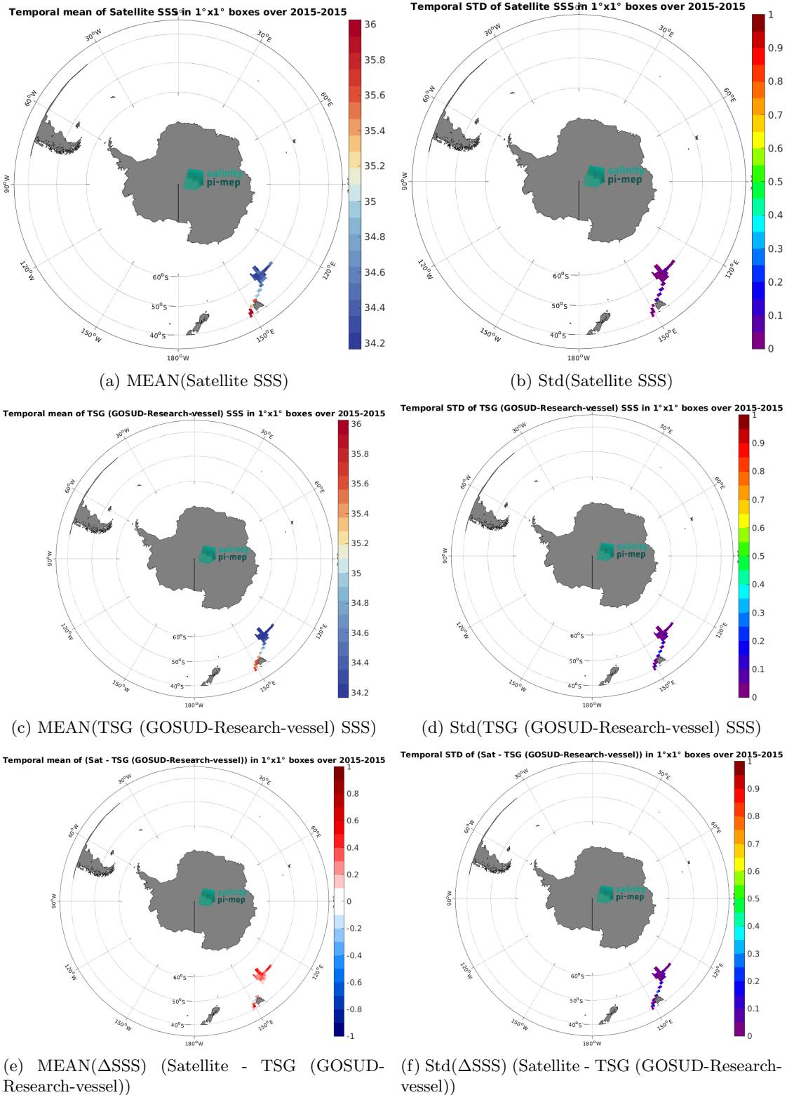
Figure 7: Temporal mean (left) and Std (right) of SSS from Aquarius SSS L3 CAP v5 - Monthly (JPL) (top), TSG (GOSUD-Research-vessel) (middle), and of \Delta SSS (Satellite - TSG (GOSUD-Research-vessel)). Only match-up pairs are used to generate these maps.
