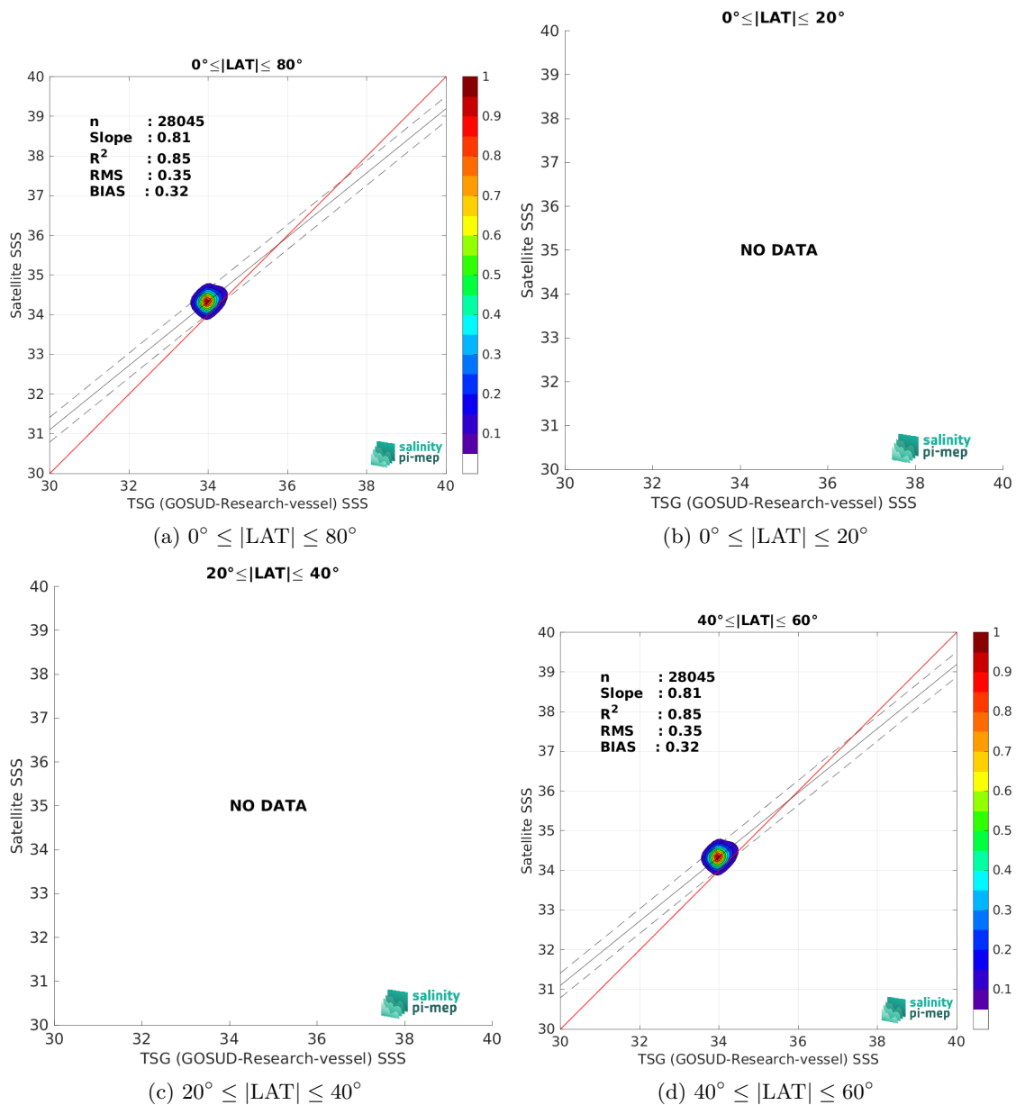
Figure 10: Contour maps of the concentration of Aquarius SSS L3 CAP v5 - Monthly (JPL) SSS (y-axis) versus TSG (GOSUD-Research-vessel) SSS (x-axis) at match-up pairs for different latitude bands. For each plot, the red line shows x=y . The black thin and dashed lines indicate a linear fit through the data cloud and the \pm 95\% confidence levels, respectively. The number match-up pairs n , the slope and R^2 coefficient of the linear fit, the root mean square (RMS) and the mean bias between satellite and in situ data are indicated for each latitude band in each plots.
