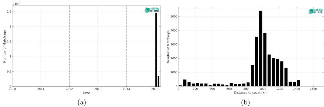
Figure 2: Number of match-ups between TSG (GOSUD-Research-vessel) and Aquarius SSS L3 CAP v5 - Monthly (JPL) SSS as a function of time (a) and as function of the distance to coast (b) over the Roaring Forties and Furious Fifties Pi-MEP region and for the full satellite product period.
