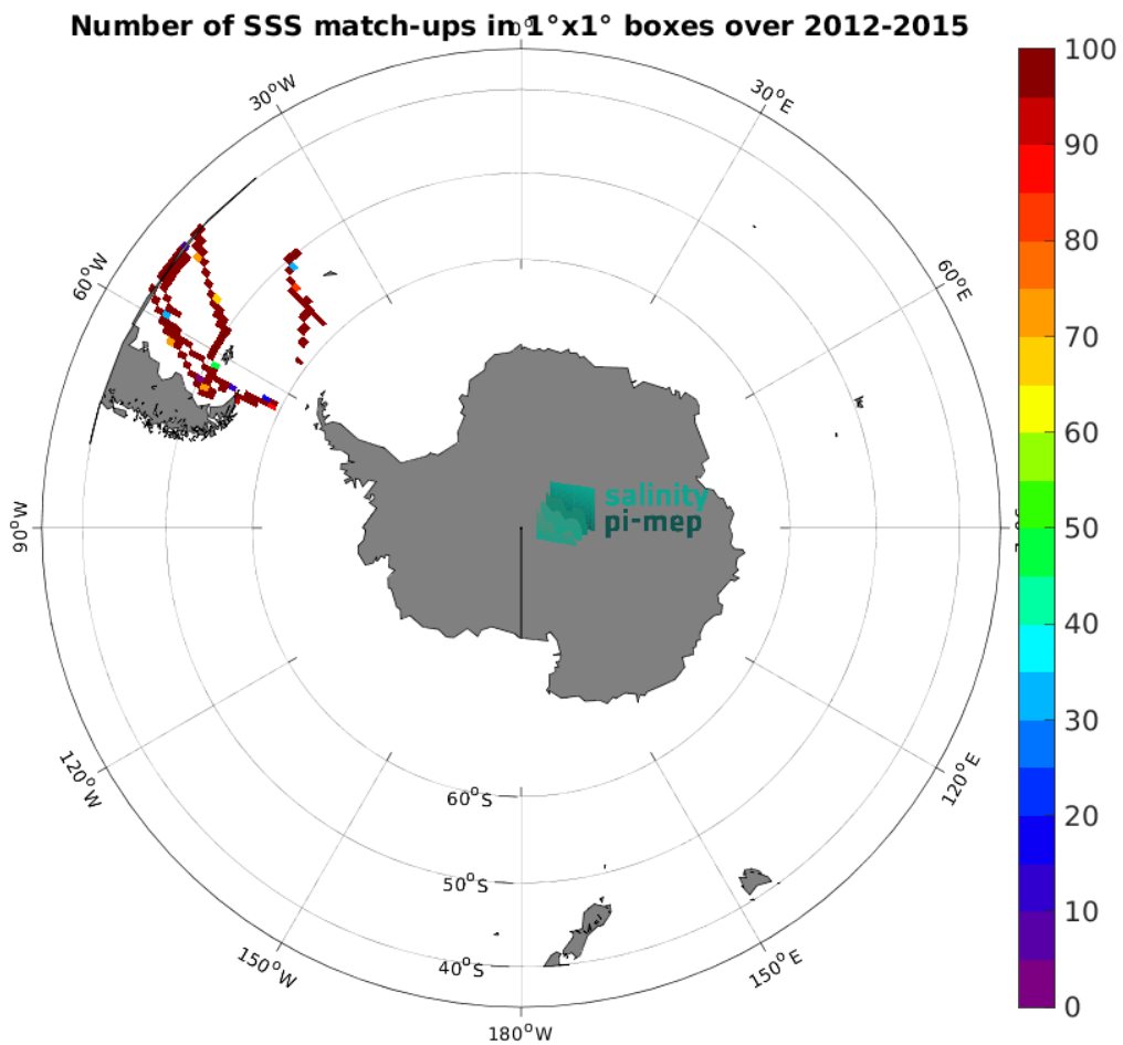
Figure 5: Number of SSS match-ups between TSG (CSIC-UTM) SSS and the Aquarius SSS L3 CAP v5 - Monthly (JPL) SSS product for the Roaring Forties and Furious Fifties Pi-MEP region over 1^\circ \times 1^\circ boxes and for the full satellite product period.
