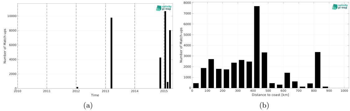
Figure 2: Number of match-ups between TSG (CSIC-UTM) and Aquarius SSS L3 CAP v5 - Monthly (JPL) SSS as a function of time (a) and as function of the distance to coast (b) over the Roaring Forties and Furious Fifties Pi-MEP region and for the full satellite product period.
