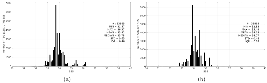
Figure 3: Histograms of SSS from TSG (CSIC-UTM) (a) and Aquarius SSS L3 CAP v5 - Monthly (JPL) (b) considering all match-up pairs per bins of 0.1 over the Roaring Forties and Furious Fifties Pi-MEP region and for the full satellite product period.
