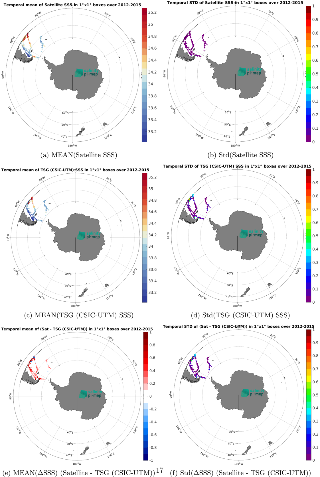
Figure 7: Temporal mean (left) and Std (right) of SSS from Aquarius SSS L3 CAP v5 - Monthly (JPL) (top), TSG (CSIC-UTM) (middle), and of \Delta SSS (Satellite - TSG (CSIC-UTM)). Only match-up pairs are used to generate these maps.
