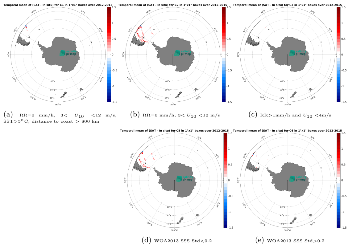
Figure 14: Temporal mean gridded over spatial boxes of size 1^\circ \times 1^\circ of \Delta\text{SSS} (Aquarius SSS L3 CAP v5 - Monthly (JPL) - TSG (CSIC-UTM)) for 5 different subdatasets corresponding to:RR=0 mm/h, 3 < U_{10} < 12 m/s, SST>5°C, distance to coast > 800 km (a), RR=0 mm/h, 3 < U_{10} < 12 m/s (b), RR>1mm/h and U_{10} < 4 m/s (c), WOA2013 SSS Std<0.2 (d), WOA2013 SSS Std>0.2 (e).
