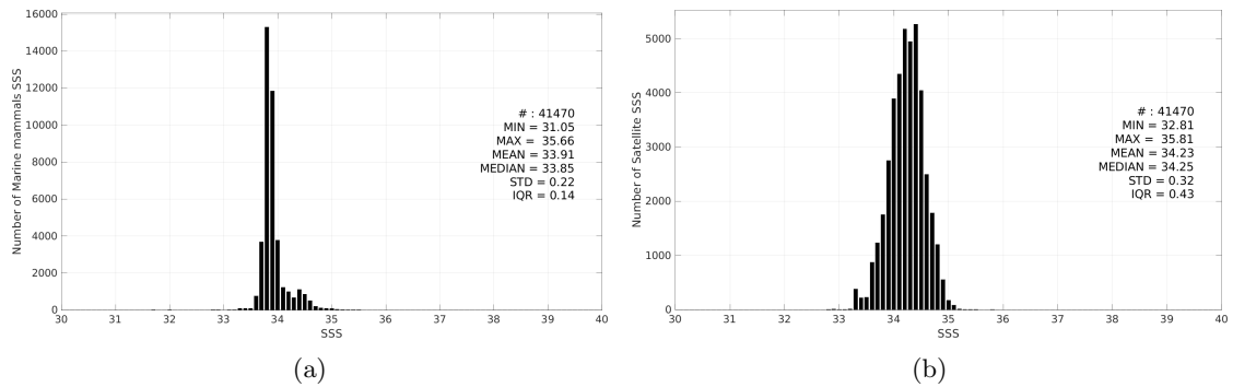
Figure 3: Histograms of SSS from Marine mammals (a) and Aquarius SSS L3 CAP v5 - Monthly (JPL) (b) considering all match-up pairs per bins of 0.1 over the Roaring Forties and Furious Fifties Pi-MEP region and for the full satellite product period.
