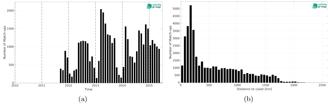
Figure 2: Number of match-ups between Marine mammals and Aquarius SSS L3 CAP v5 - Monthly (JPL) SSS as a function of time (a) and as function of the distance to coast (b) over the Roaring Forties and Furious Fifties Pi-MEP region and for the full satellite product period.
