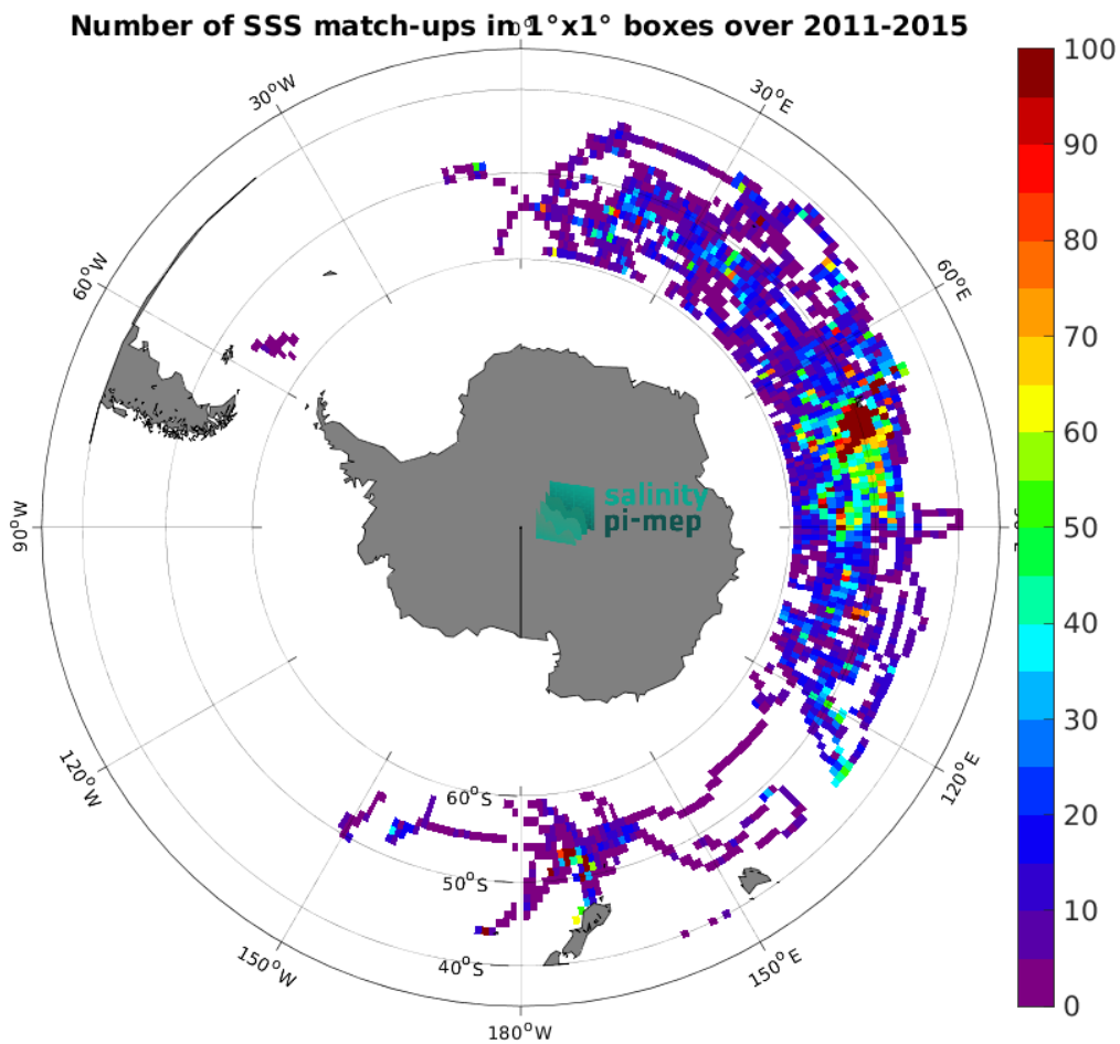
Figure 5: Number of SSS match-ups between Marine mammals SSS and the Aquarius SSS L3 CAP v5 - Monthly (JPL) SSS product for the Roaring Forties and Furious Fifties Pi-MEP region over 1^{\circ} \times 1^{\circ} boxes and for the full satellite product period.
