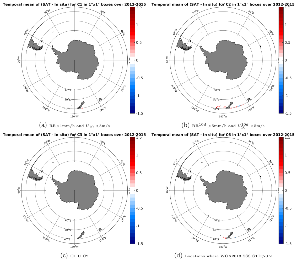
Figure 12: Temporal mean gridded over spatial boxes of size 1^\circ \times 1^\circ of \Delta SSS (Aquarius-L3-JPL-V4-7DAY-RUNNING - TSG-LEGOS-DM) for 4 different subdatasets corresponding to: RR > 1\text{mm/h} and U_{10} < 5\text{m/s} (a), RR^{10d} > 5\text{mm/h} and U_{10}^{10d} < 5\text{m/s} (b), C1 U C2 (c), Locations where WOA2013 SSS STD > 0.2 (d).
