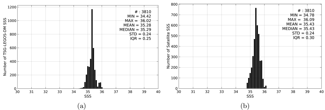
Figure 2: Histograms of SSS from TSG-LEGOS-DM (a) and Aquarius-L3-JPL-V4-7DAY-RUNNING (b) considering all match-up pairs per bins of 0.1 over the Roaring Forties and Furious Fifties Pi-MEP region and for the full satellite product period.
