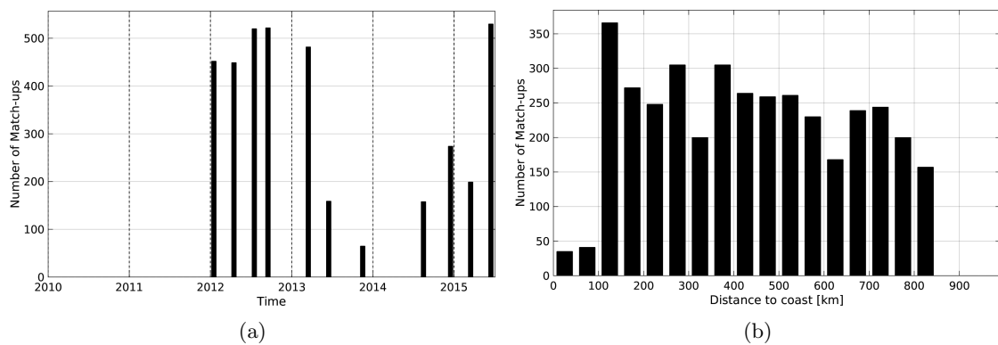
Figure 1: Number of match-ups between TSG-LEGOS-DM and Aquarius-L3-JPL-V4-7DAY-RUNNING SSS as a function of time (a) and as function of the distance to coast (b) over the Roaring Forties and Furious Fifties Pi-MEP region and for the full satellite product period.
