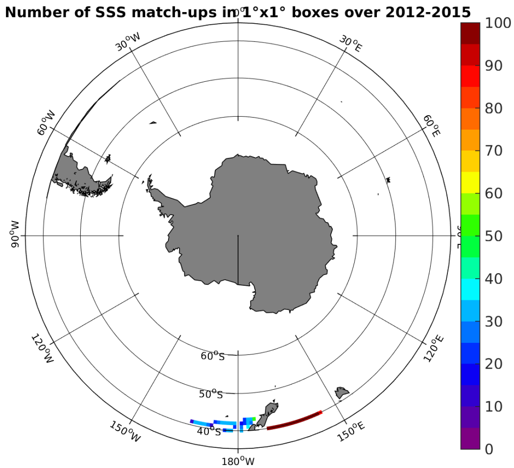
Figure 4: Number of SSS match-ups between TSG-LEGOS-DM SSS and the Aquarius-L3-JPL-V4-7DAY-RUNNING SSS product for the Roaring Forties and Furious Fifties Pi-MEP region over 1^\circ \times 1^\circ boxes and for the full satellite product period.
