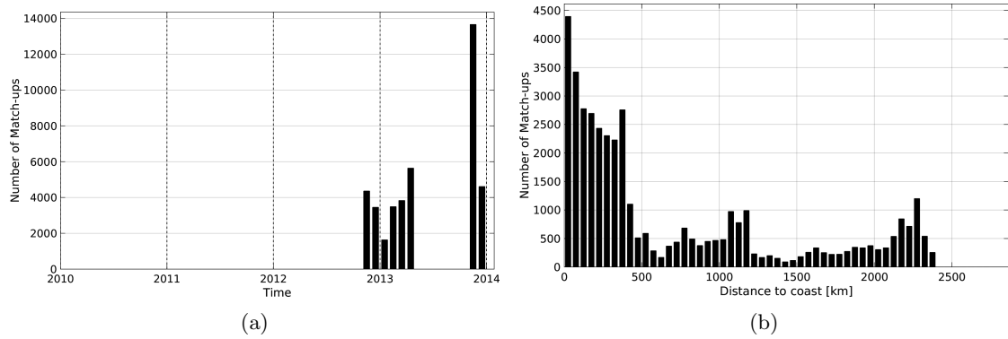
Figure 1: Number of match-ups between TSG-GOSUD-Sailing-ship and Aquarius-L3-JPL-V4-MONTHLY SSS as a function of time (a) and as function of the distance to coast (b) over the Roaring Forties and Furious Fifties Pi-MEP region and for the full satellite product period.
