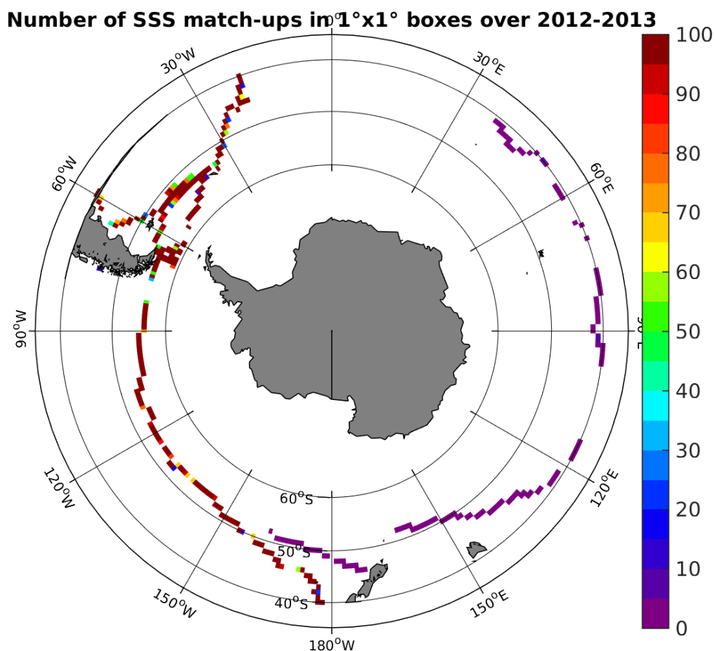
Figure 4: Number of SSS match-ups between TSG-GOSUD-Sailing-ship SSS and the Aquarius-L3-JPL-V4-MONTHLY SSS product for the Roaring Forties and Furious Fifties Pi-MEP region over 1^\circ \times 1^\circ boxes and for the full satellite product period.
