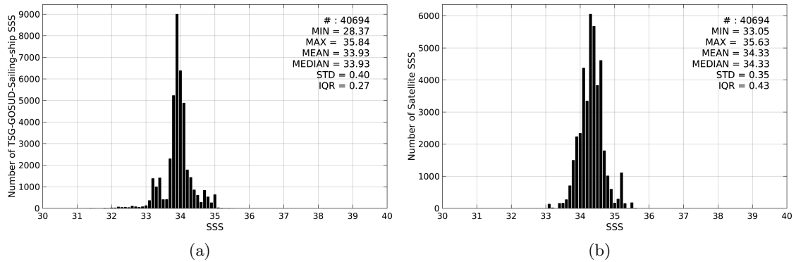
Figure 2: Histograms of SSS from TSG-GOSUD-Sailing-ship (a) and Aquarius-L3-JPL-V4-MONTHLY (b) considering all match-up pairs per bins of 0.1 over the Roaring Forties and Furious Fifties Pi-MEP region and for the full satellite product period.
