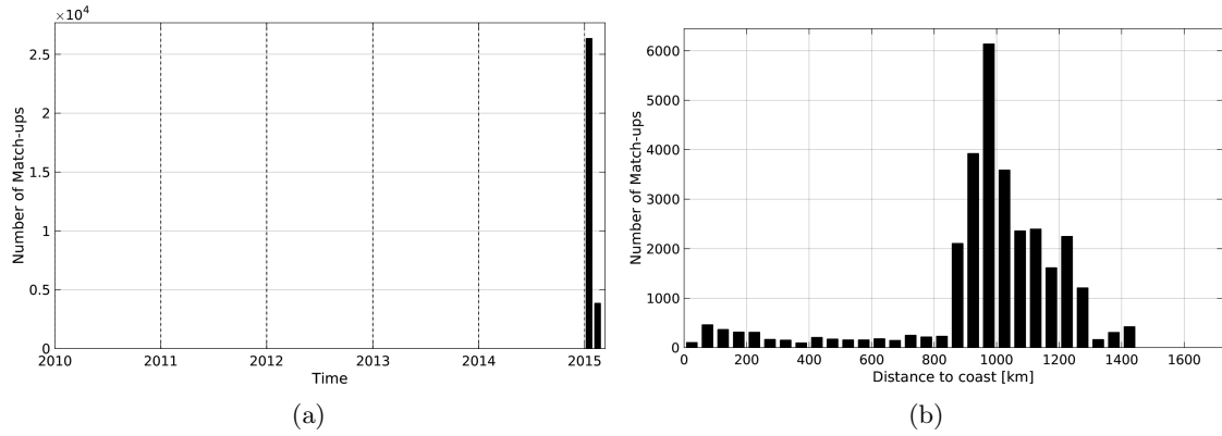
Figure 1: Number of match-ups between TSG-GOSUD-Research-vessel and Aquarius-L3-JPL-V4-MONTHLY SSS as a function of time (a) and as function of the distance to coast (b) over the Roaring Forties and Furious Fifties Pi-MEP region and for the full satellite product period.
