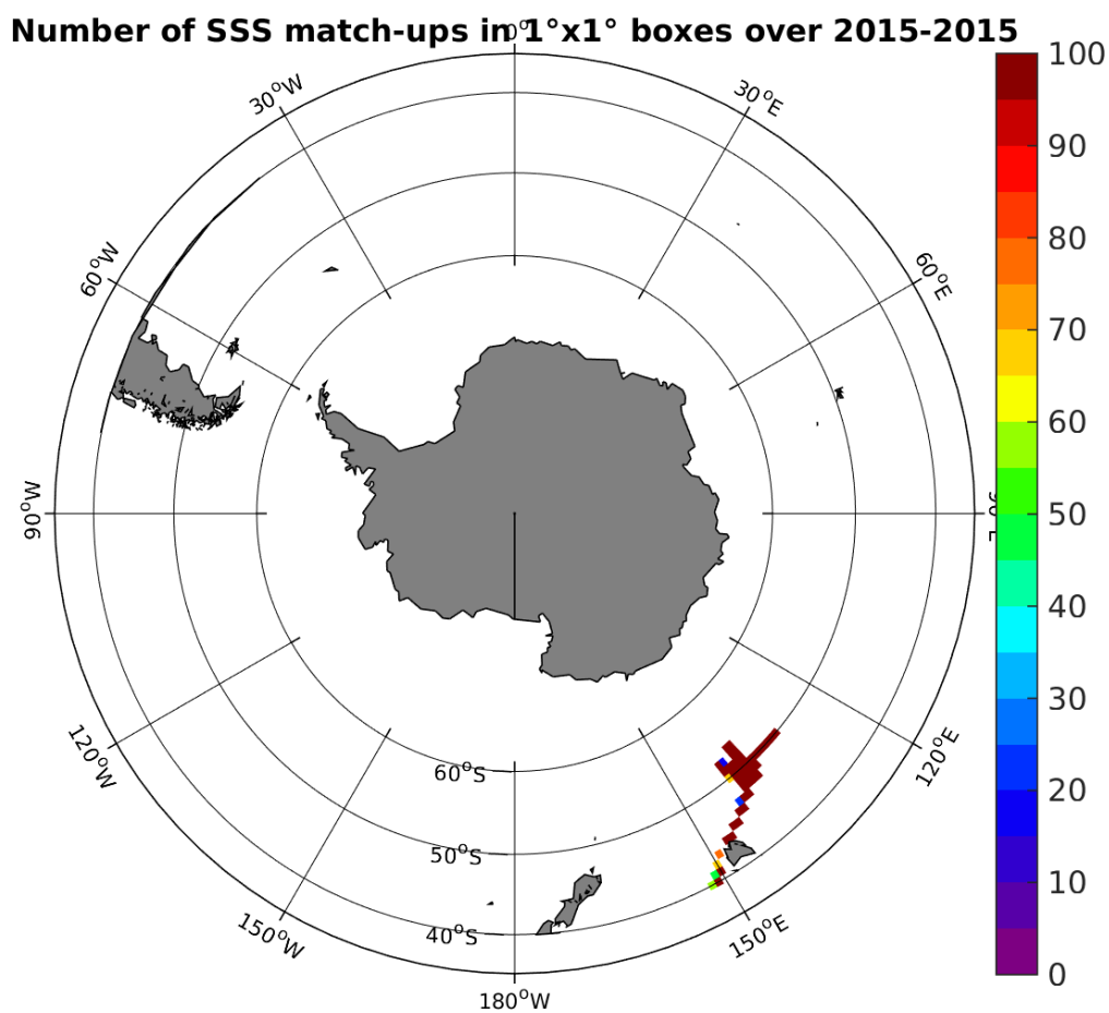
Figure 4: Number of SSS match-ups between TSG-GOSUD-Research-vessel SSS and the Aquarius-L3-JPL-V4-MONTHLY SSS product for the Roaring Forties and Furious Fifties Pi-MEP region over 1^\circ \times 1^\circ boxes and for the full satellite product period.
