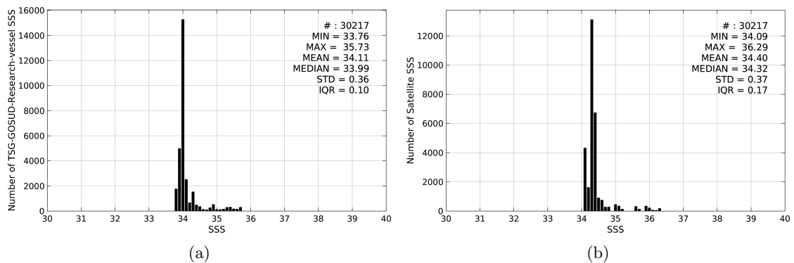
Figure 2: Histograms of SSS from TSG-GOSUD-Research-vessel (a) and Aquarius-L3-JPL-V4-MONTHLY (b) considering all match-up pairs per bins of 0.1 over the Roaring Forties and Furious Fifties Pi-MEP region and for the full satellite product period.
