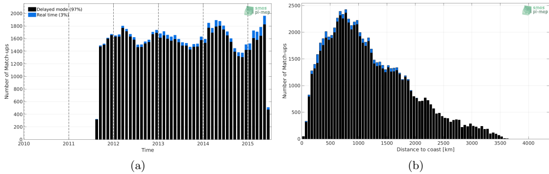
Figure 1: Number of match-ups between Argo and Aquarius SSS L2-AVERAGED OR v5 (NASA-GSFC) SSS as a function of time (a) and as function of the distance to coast (b) over the Roaring Forties and Furious Fifties Pi-MEP region and for the full satellite product period.
