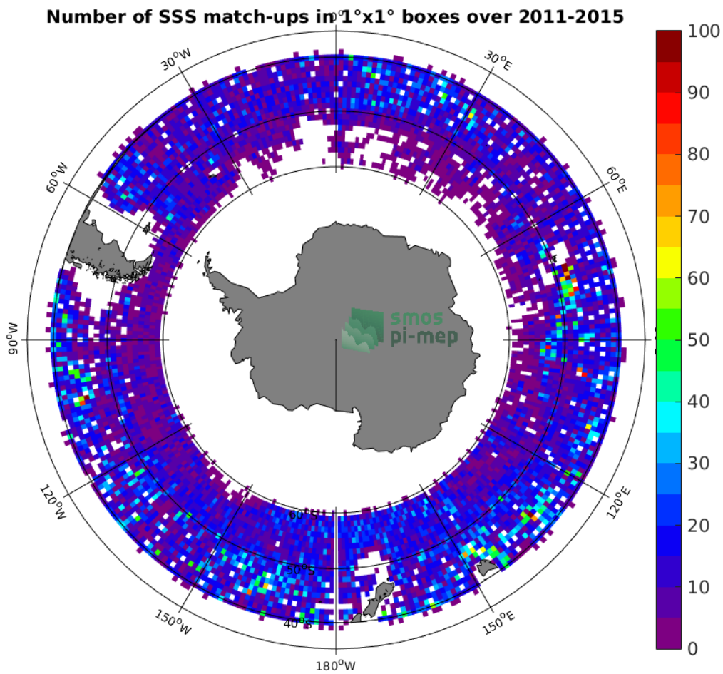
Figure 4: Number of SSS match-ups between Argo SSS and the Aquarius SSS L2-AVERAGED OR v5 (NASA-GSFC) SSS product for the Roaring Forties and Furious Fifties Pi-MEP region over 1^\circ \times 1^\circ boxes and for the full satellite product period.
