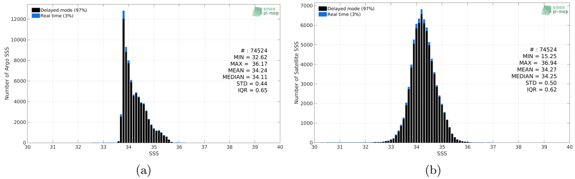
Figure 2: Histograms of SSS from Argo (a) and Aquarius SSS L2-AVERAGED OR v5 (NASA-GSFC) (b) considering all match-up pairs per bins of 0.1 over the Roaring Forties and Furious Fifties Pi-MEP region and for the full satellite product period.
