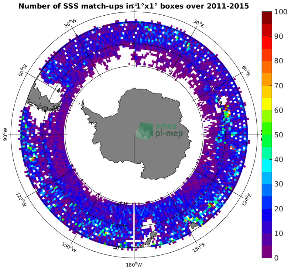
Figure 4: Number of SSS match-ups between Argo SSS and the Aquarius SSS L2-AVERAGED CAP v5 (JPL) SSS product for the Roaring Forties and Furious Fifties Pi-MEP region over 1^\circ \times 1^\circ boxes and for the full satellite product period.
