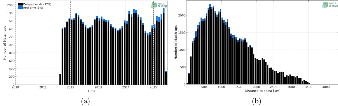
Figure 1: Number of match-ups between Argo and Aquarius SSS L2-AVERAGED CAP v5 (JPL) SSS as a function of time (a) and as function of the distance to coast (b) over the Roaring Forties and Furious Fifties Pi-MEP region and for the full satellite product period.
