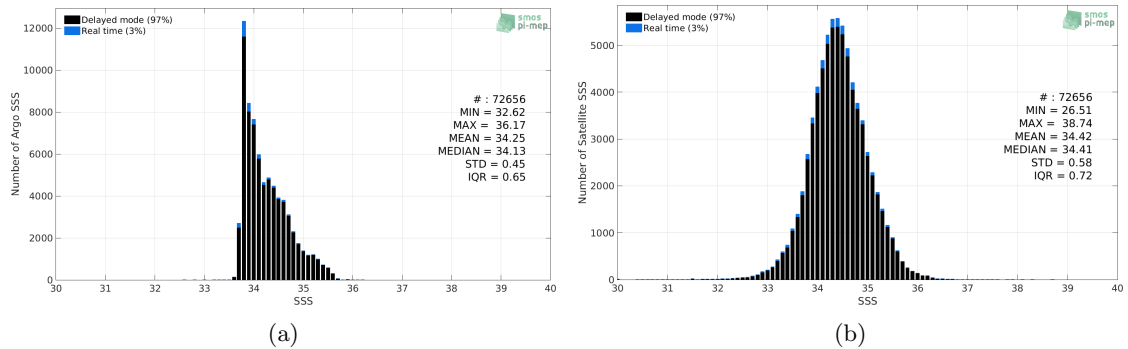
Figure 2: Histograms of SSS from Argo (a) and Aquarius SSS L2-AVERAGED CAP v5 (JPL) (b) considering all match-up pairs per bins of 0.1 over the Roaring Forties and Furious Fifties Pi-MEP region and for the full satellite product period.
