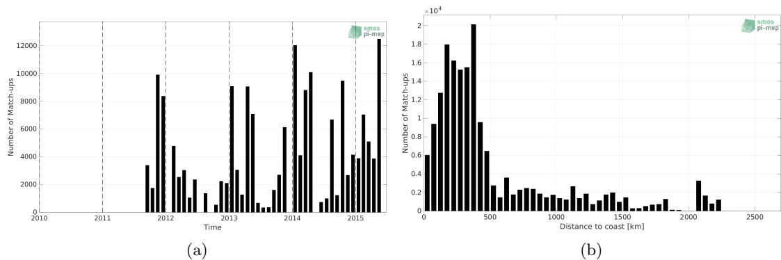
Figure 1: Number of match-ups between TSG (SAMOS) and Aquarius SSS L2 OR v5 (NASA-GSFC) SSS as a function of time (a) and as function of the distance to coast (b) over the Roaring Forties and Furious Fifties Pi-MEP region and for the full satellite product period.
