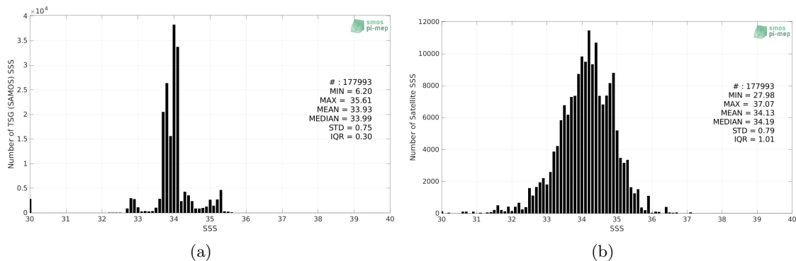
Figure 2: Histograms of SSS from TSG (SAMOS) (a) and Aquarius SSS L2 OR v5 (NASA-GSFC) (b) considering all match-up pairs per bins of 0.1 over the Roaring Forties and Furious Fifties Pi-MEP region and for the full satellite product period.
