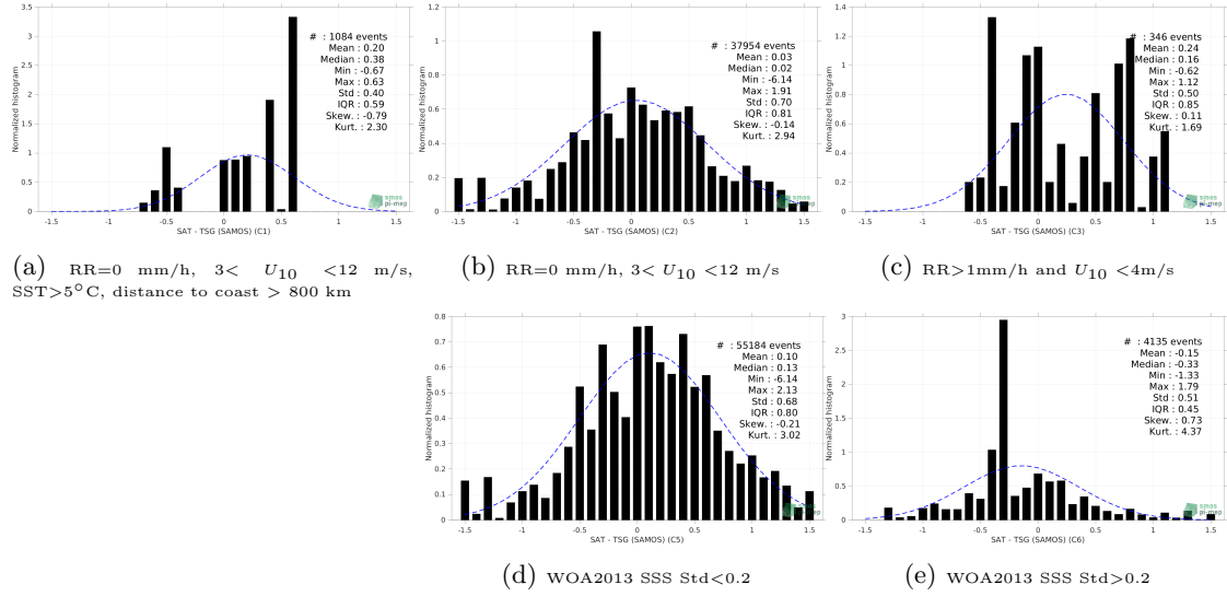
Figure 13: Normalized histogram of \Delta SSS (Aquarius SSS L2 OR v5 (NASA-GSFC) - TSG (SAMOS)) for 5 different subdatasets corresponding to: RR=0 mm/h, 3 < U_{10} < 12 m/s, SST > 5°C, distance to coast > 800 km (a), RR=0 mm/h, 3 < U_{10} < 12 m/s (b), RR > 1mm/h and U_{10} < 4 m/s (c), WOA2013 SSS Std < 0.2 (d), WOA2013 SSS Std > 0.2 (e).
