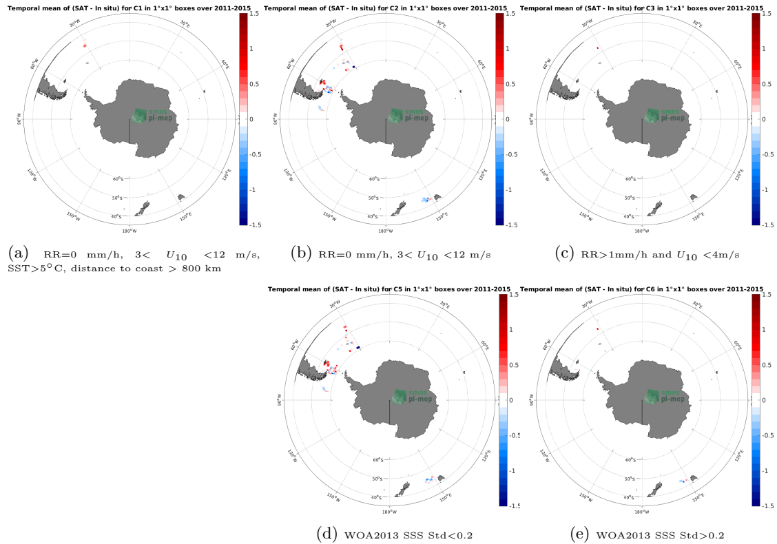
Figure 12: Temporal mean gridded over spatial boxes of size 1^{\circ}\times 1^{\circ} of \Delta\text{SSS} (Aquarius SSS L2 OR v5 (NASA-GSFC) - TSG (SAMOS)) for 5 different subdatasets corresponding to:RR=0 mm/h, 3 < U_{10} < 12 m/s, SST >5^{\circ}\text{C} , distance to coast > 800 km (a), RR=0 mm/h, 3 < U_{10} < 12 m/s (b), RR >1 mm/h and U_{10} < 4 m/s (c), WOA2013 SSS Std <0.2 (d), WOA2013 SSS Std >0.2 (e).
