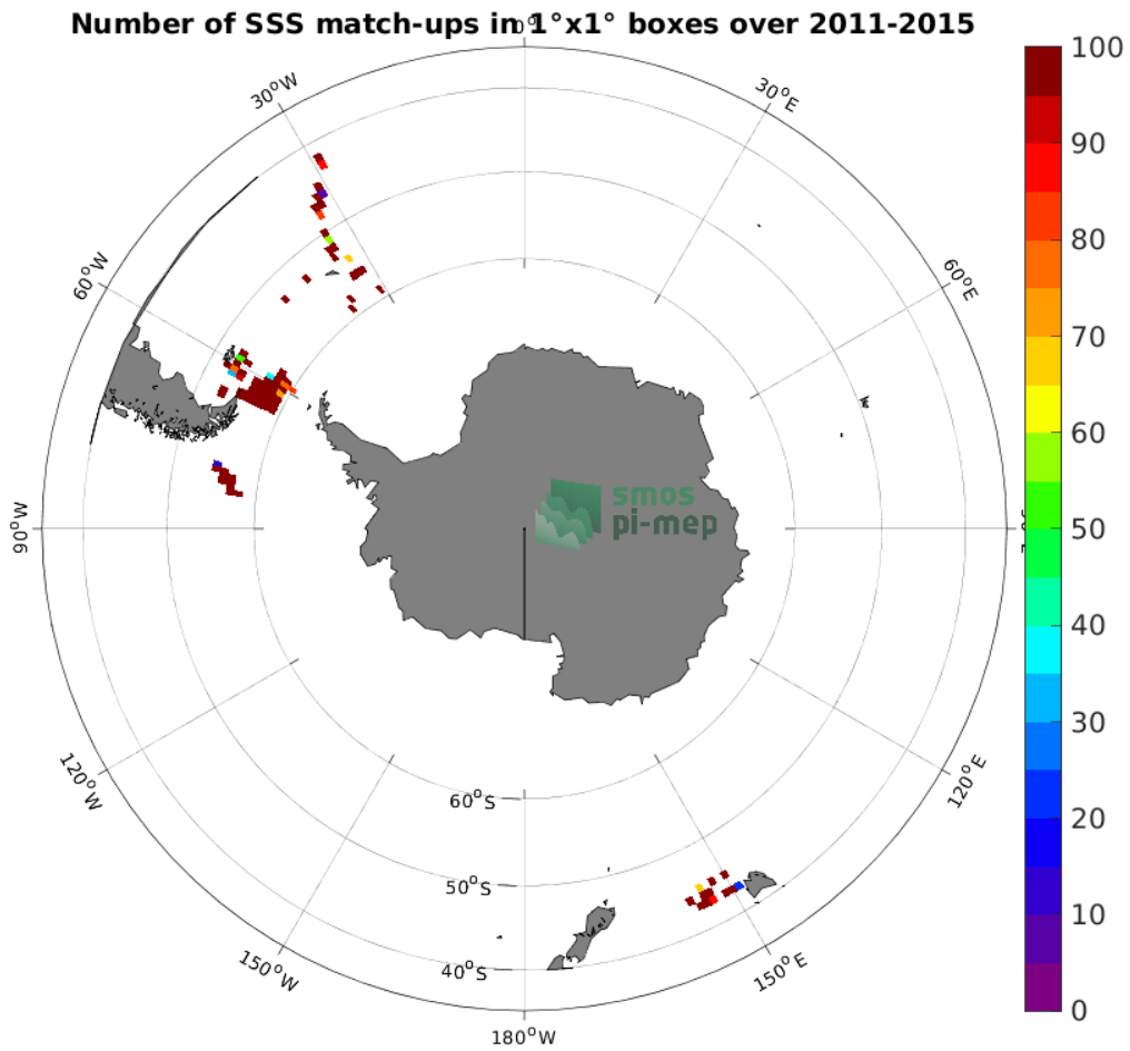
Figure 4: Number of SSS match-ups between TSG (SAMOS) SSS and the Aquarius SSS L2 OR v5 (NASA-GSFC) SSS product for the Roaring Forties and Furious Fifties Pi-MEP region over 1^\circ \times 1^\circ boxes and for the full satellite product period.
