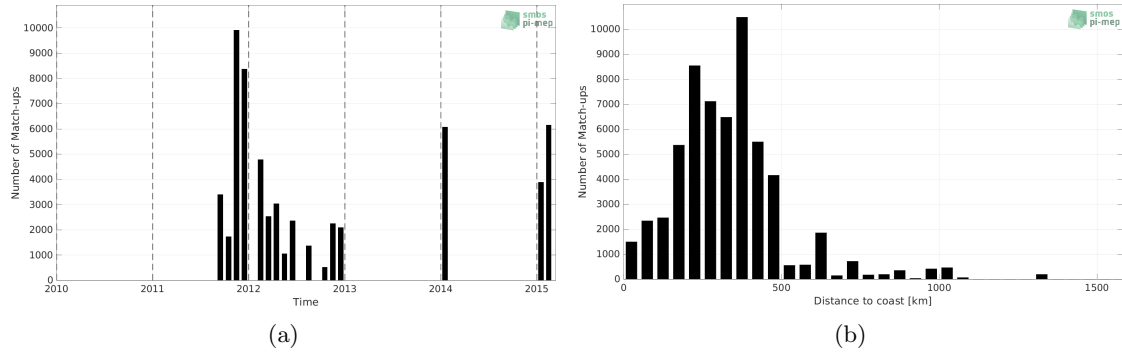
Figure 1: Number of match-ups between TSG (SAMOS) and Aquarius SSS L2 OR v5 (NASA-GSFC) SSS as a function of time (a) and as function of the distance to coast (b) over the Roaring Forties and Furious Fifties Pi-MEP region and for the full satellite product period.
