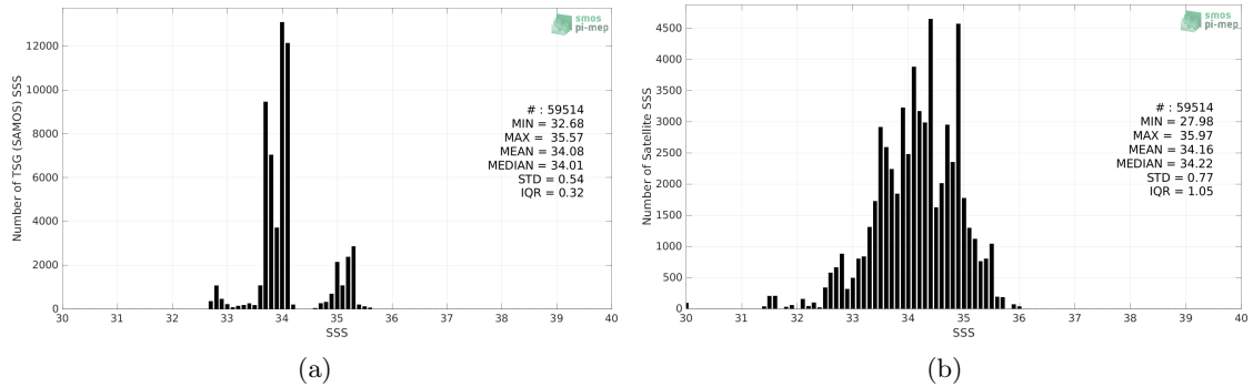
Figure 2: Histograms of SSS from TSG (SAMOS) (a) and Aquarius SSS L2 OR v5 (NASA-GSFC) (b) considering all match-up pairs per bins of 0.1 over the Roaring Forties and Furious Fifties Pi-MEP region and for the full satellite product period.
