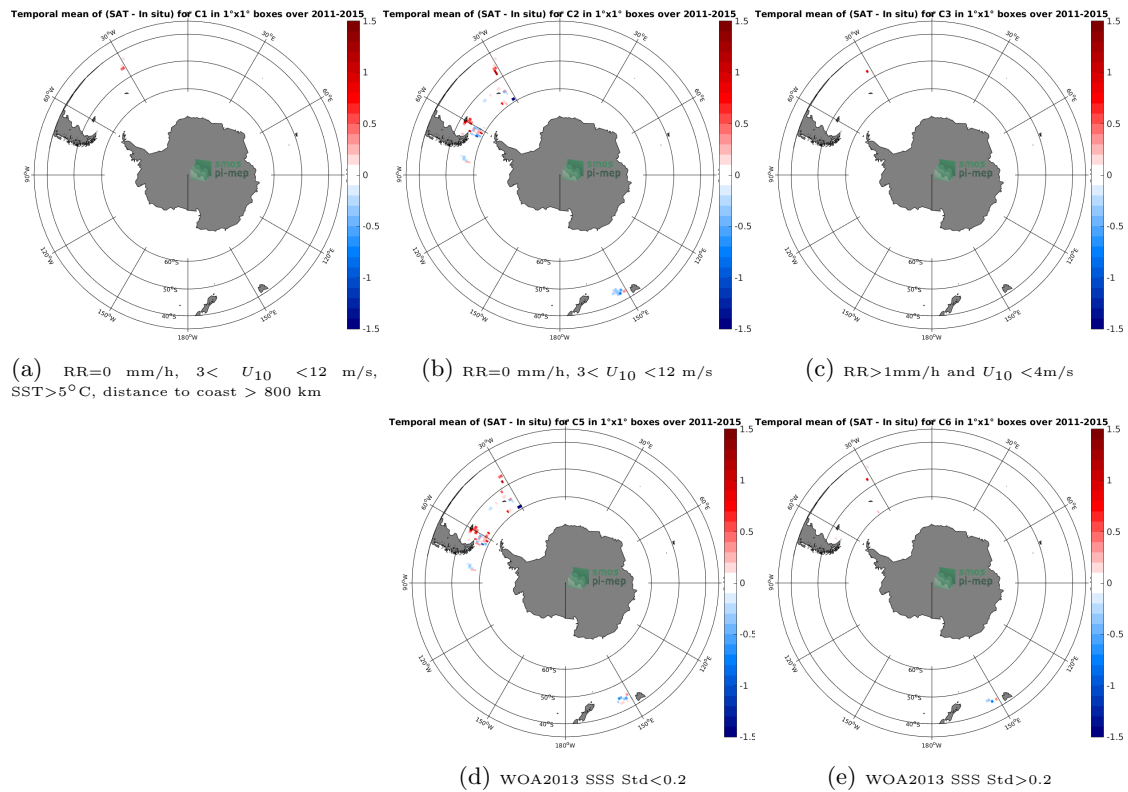
Figure 12: Temporal mean gridded over spatial boxes of size 1^{\circ}\times 1^{\circ} of \Delta\text{SSS} (Aquarius-L2-OR-V5 - TSG-SAMOS) for 5 different subdatasets corresponding to:RR=0 mm/h, 3 < U_{10} < 12 m/s, SST > 5^{\circ}\text{C} , distance to coast > 800 km (a), RR=0 mm/h, 3 < U_{10} < 12 m/s (b), RR > 1 mm/h and U_{10} < 4 m/s (c), WOA2013 SSS Std < 0.2 (d), WOA2013 SSS Std > 0.2 (e).
