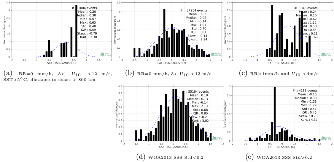
Figure 13: Normalized histogram of \Delta SSS (Aquarius-L2-OR-V5 - TSG-SAMOS) for 5 different subdatasets corresponding to: RR=0 mm/h, 3 < U_{10} < 12 m/s, SST>5°C, distance to coast > 800 km (a), RR=0 mm/h, 3 < U_{10} < 12 m/s (b), RR>1mm/h and U_{10} < 4 m/s (c), WOA2013 SSS Std<0.2 (d), WOA2013 SSS Std>0.2 (e).
