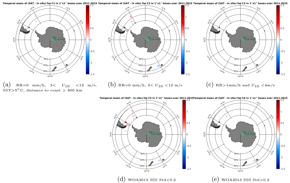
Figure 12: Temporal mean gridded over spatial boxes of size 1^\circ \times 1^\circ of \Delta SSS (Aquarius-L2-OR-V5 - TSG-SAMOS) for 5 different subdatasets corresponding to: RR=0 mm/h, 3 < U_{10} < 12 m/s, SST > 5^\circ\text{C} , distance to coast > 800 km (a), RR=0 mm/h, 3 < U_{10} < 12 m/s (b), RR > 1 mm/h and U_{10} < 4 m/s (c), WOA2013 SSS Std < 0.2 (d), WOA2013 SSS Std > 0.2 (e).
