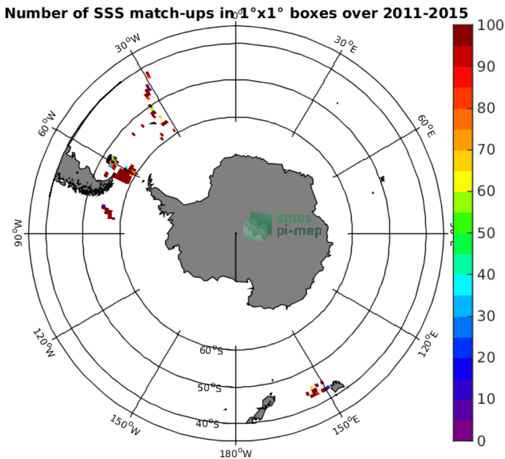
Figure 4: Number of SSS match-ups between TSG-SAMOS SSS and the Aquarius-L2-OR-V5 SSS product for the Roaring Forties and Furious Fifties Pi-MEP region over 1°x1° boxes and for the full satellite product period.
