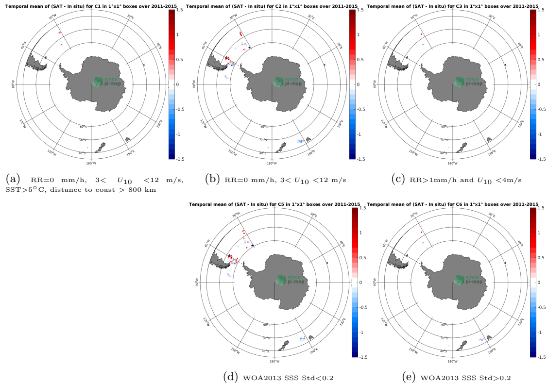
Figure 12: Temporal mean gridded over spatial boxes of size 1^\circ \times 1^\circ of \Delta SSS (Aquarius-L2-OR-V5 - TSG-SAMOS) for 5 different subdatasets corresponding to:RR=0 mm/h, 3 < U_{10} < 12 m/s, SST >5^\circ C, distance to coast > 800 km (a), RR=0 mm/h, 3 < U_{10} < 12 m/s (b), RR >1 mm/h and U_{10} < 4 m/s (c), WOA2013 SSS Std <0.2 (d), WOA2013 SSS Std >0.2 (e).
