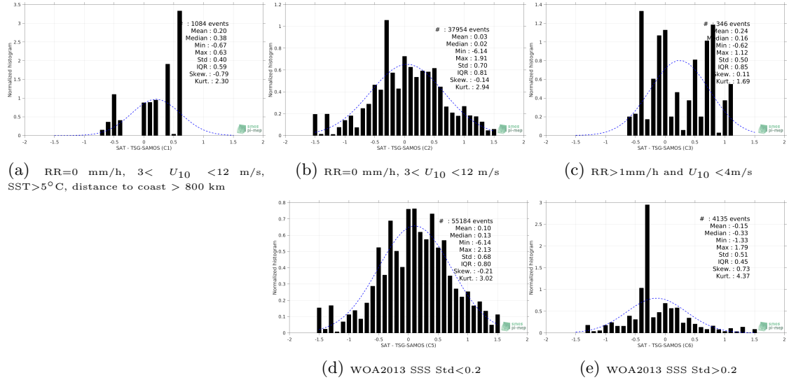
Figure 13: Normalized histogram of \Delta SSS (Aquarius-L2-OR-V5 - TSG-SAMOS) for 5 different subdatasets corresponding to: RR=0 mm/h, 3 < U_{10} < 12 m/s, SST > 5°C, distance to coast > 800 km (a), RR=0 mm/h, 3 < U_{10} < 12 m/s (b), RR > 1mm/h and U_{10} < 4 m/s (c), WOA2013 SSS Std < 0.2 (d), WOA2013 SSS Std > 0.2 (e).
