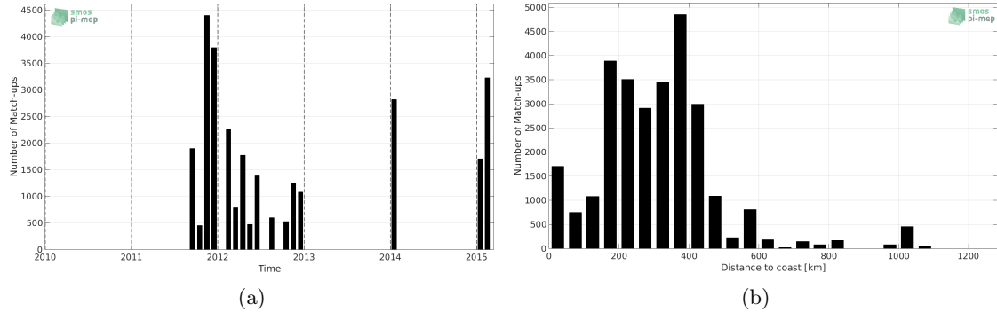
Figure 1: Number of match-ups between TSG-SAMOS and Aquarius-L2-OR-V5 SSS as a function of time (a) and as function of the distance to coast (b) over the Roaring Forties and Furious Fifties Pi-MEP region and for the full satellite product period.
