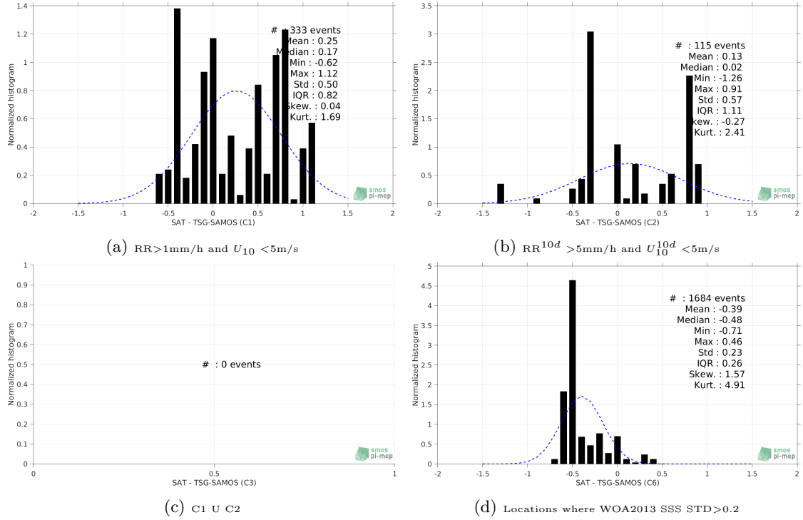
Figure 13: Normalized histogram of \Delta SSS (Aquarius-L2-OR-V5 - TSG-SAMOS) for 6 different subdatasets corresponding to: RR > 1\text{mm/h} and U_{10} < 5\text{m/s} (a), RR^{10d} > 5\text{mm/h} and U_{10}^{10d} < 5\text{m/s} (b), C1 \cup C2 (c), Locations where WOA2013 SSS STD > 0.2 (d).
