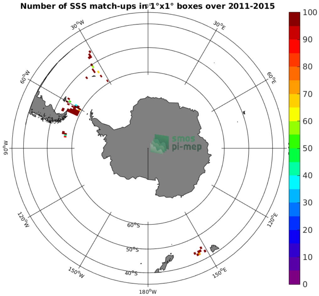
Figure 4: Number of SSS match-ups between TSG-SAMOS SSS and the Aquarius-L2-OR-V5 SSS product for the Roaring Forties and Furious Fifties Pi-MEP region over 1^\circ \times 1^\circ boxes and for the full satellite product period.
