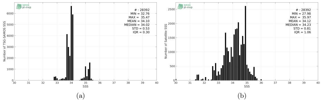
Figure 2: Histograms of SSS from TSG-SAMOS (a) and Aquarius-L2-OR-V5 (b) considering all match-up pairs per bins of 0.1 over the Roaring Forties and Furious Fifties Pi-MEP region and for the full satellite product period.
