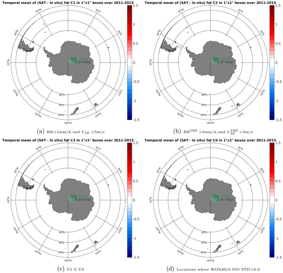
Figure 12: Temporal mean gridded over spatial boxes of size 1^\circ \times 1^\circ of \Delta SSS (Aquarius-L2-OR-V5 - TSG-SAMOS) for 4 different subdatasets corresponding to:RR >1 mm/h and U_{10} < 5 m/s (a), RR 10d > 5 mm/h and U_{10}^{10d} < 5 m/s (b), C1 U C2 (c),Locations where WOA2013 SSS STD >0.2 (d).
