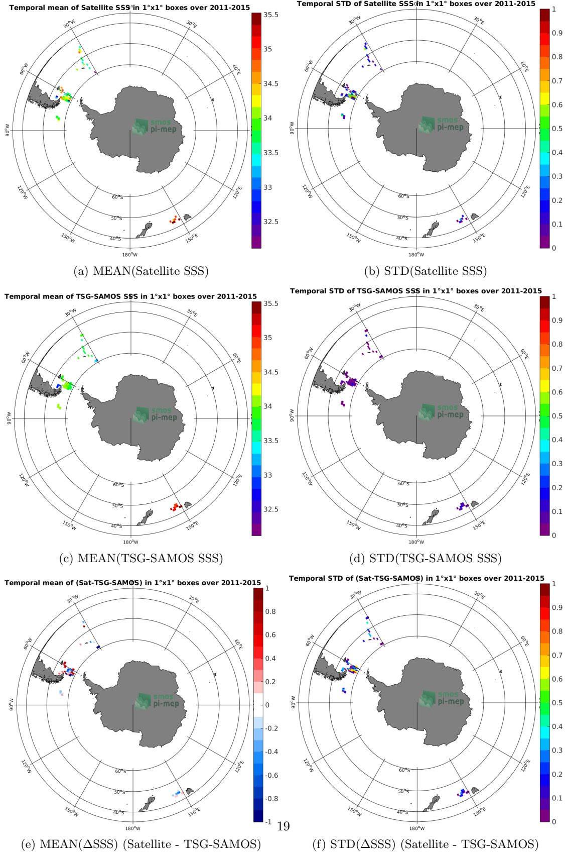
Figure 6: Temporal mean (left) and STD (right) of SSS from Aquarius-L2-OR-V5 (top), TSG-SAMOS (middle), and of \Delta SSS (Satellite - TSG-SAMOS). Only match-up pairs are used to generate these maps.
