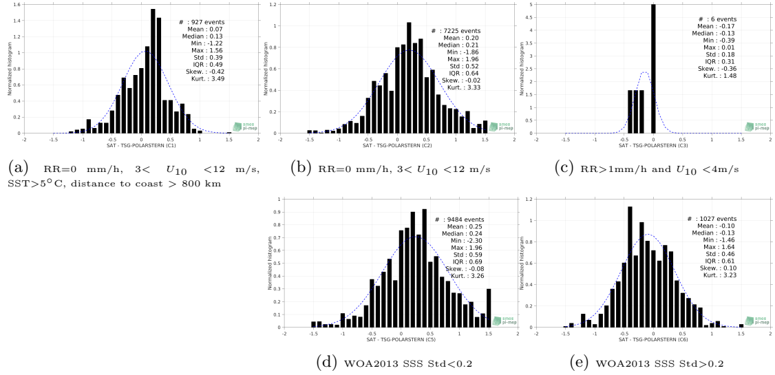
Figure 13: Normalized histogram of \Delta SSS (Aquarius-L2-OR-V5 - TSG-POLARSTERN) for 5 different subdatasets corresponding to: RR=0 mm/h, 3 < U_{10} < 12 m/s, SST > 5°C, distance to coast > 800 km (a), RR=0 mm/h, 3 < U_{10} < 12 m/s (b), RR > 1mm/h and U_{10} < 4 m/s (c), WOA2013 SSS Std < 0.2 (d), WOA2013 SSS Std > 0.2 (e).
