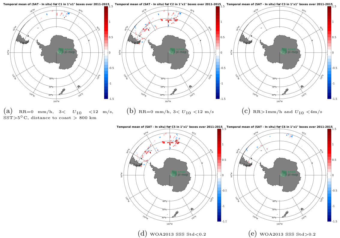
Figure 12: Temporal mean gridded over spatial boxes of size 1^{\circ}\times 1^{\circ} of \Delta\text{SSS} (Aquarius-L2-OR-V5 - TSG-POLARSTERN) for 5 different subdatasets corresponding to:RR=0 mm/h, 3 < U_{10} < 12 m/s, SST >5^{\circ}\text{C} , distance to coast > 800 km (a), RR=0 mm/h, 3 < U_{10} < 12 m/s (b), RR >1 mm/h and U_{10} < 4 m/s (c), WOA2013 SSS Std <0.2 (d), WOA2013 SSS Std >0.2 (e).
