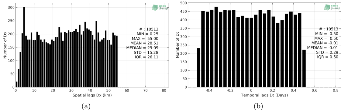
Figure 5: Histograms of the spatial (a) and temporal (b) lags between the time of the TSG-POLARSTERN measurements and the date of the corresponding Aquarius-L2-OR-V5 SSS product.
