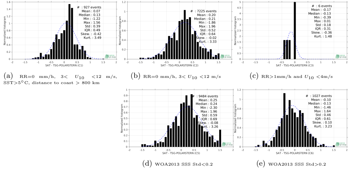
Figure 13: Normalized histogram of \Delta\text{SSS} (Aquarius-L2-OR-V5 - TSG-POLARSTERN) for 5 different subdatasets corresponding to: RR=0 mm/h, 3 < U_{10} < 12 m/s, SST>5°C, distance to coast > 800 km (a), RR=0 mm/h, 3 < U_{10} < 12 m/s (b), RR>1mm/h and U_{10} < 4 m/s (c), WOA2013 SSS Std<0.2 (d), WOA2013 SSS Std>0.2 (e).
