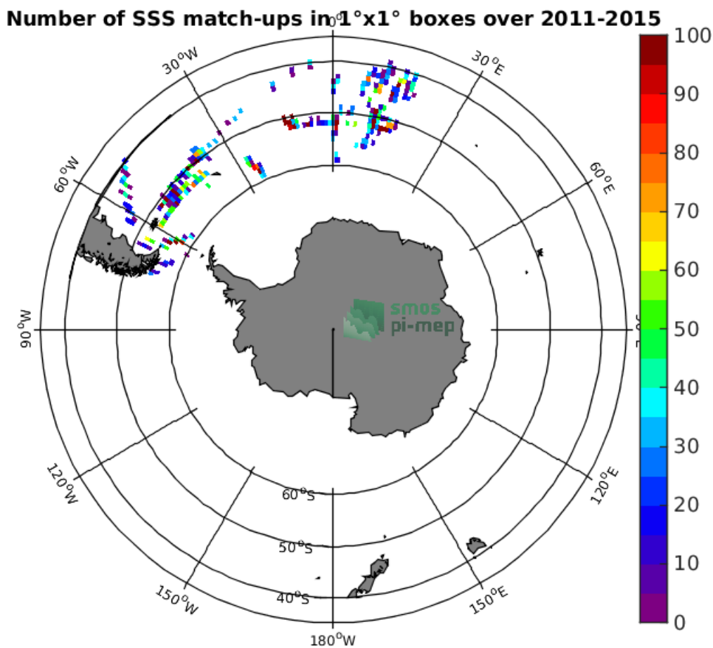
Figure 4: Number of SSS match-ups between TSG-POLARSTERN SSS and the Aquarius-L2-OR-V5 SSS product for the Roaring Forties and Furious Fifties Pi-MEP region over 1°x1° boxes and for the full satellite product period.
