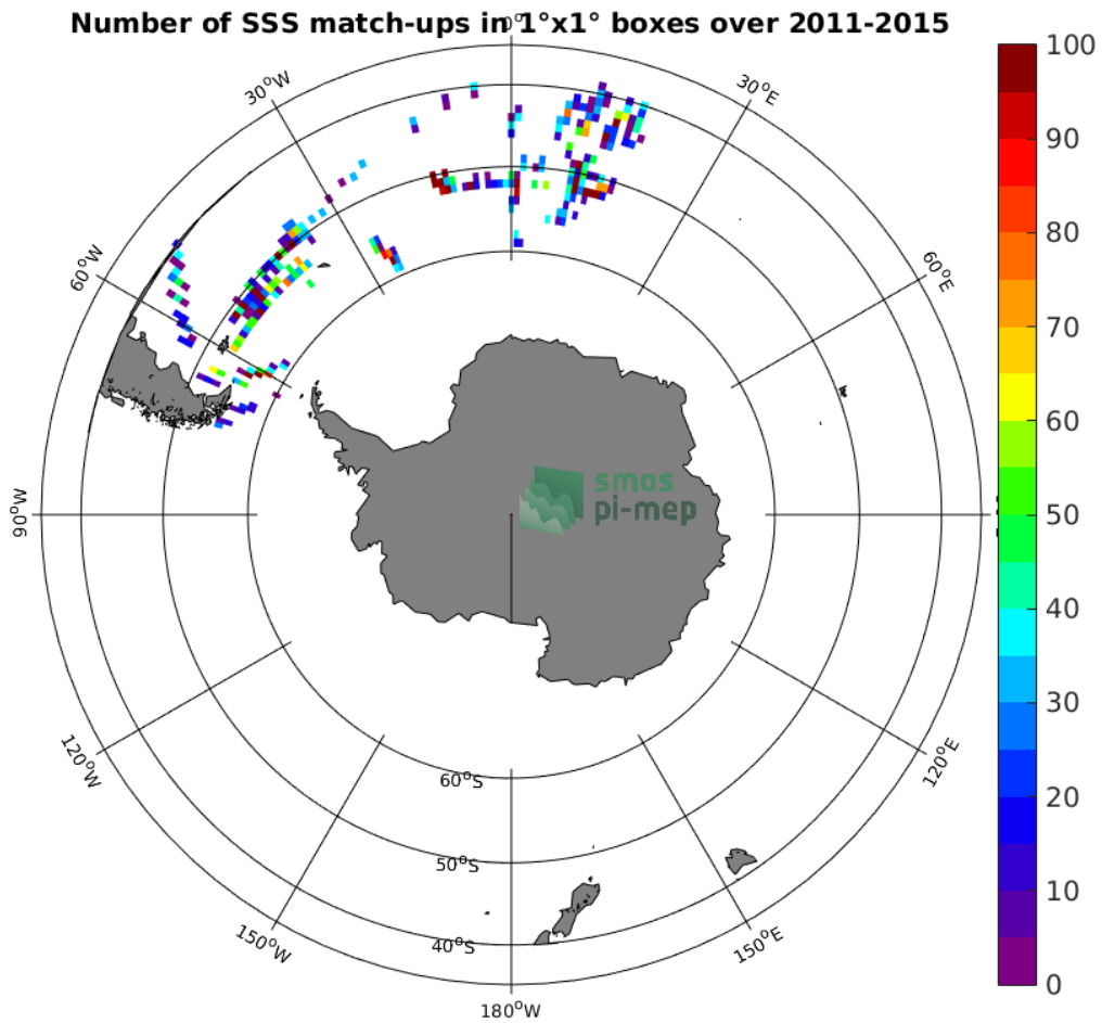
Figure 4: Number of SSS match-ups between TSG-POLARSTERN SSS and the Aquarius-L2-OR-V5 SSS product for the Roaring Forties and Furious Fifties Pi-MEP region over 1^\circ \times 1^\circ boxes and for the full satellite product period.
