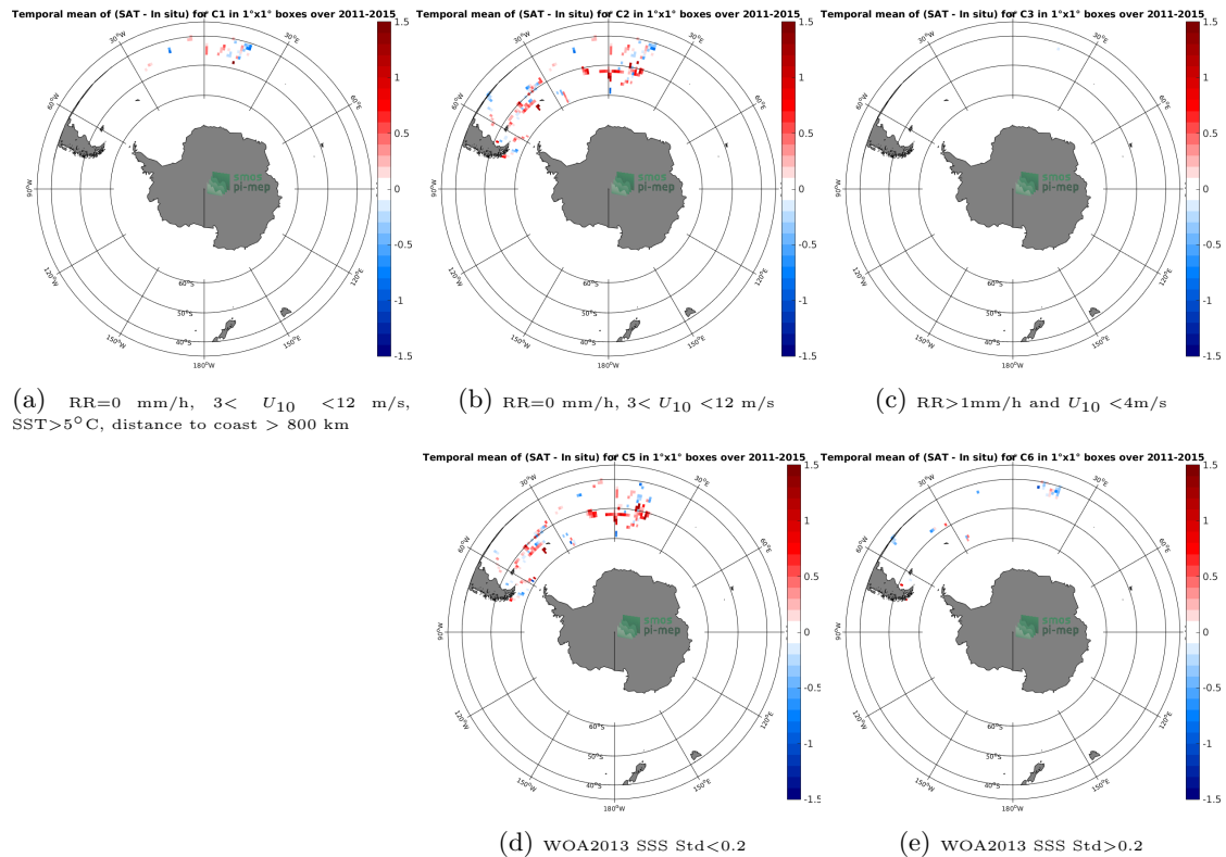
Figure 12: Temporal mean gridded over spatial boxes of size 1^\circ \times 1^\circ of \Delta SSS (Aquarius-L2-OR-V5 - TSG-POLARSTERN) for 5 different subdatasets corresponding to:RR=0 mm/h, 3 < U_{10} < 12 m/s, SST >5^\circ C, distance to coast > 800 km (a), RR=0 mm/h, 3 < U_{10} < 12 m/s (b), RR >1 mm/h and U_{10} < 4 m/s (c), WOA2013 SSS Std <0.2 (d), WOA2013 SSS Std >0.2 (e).
