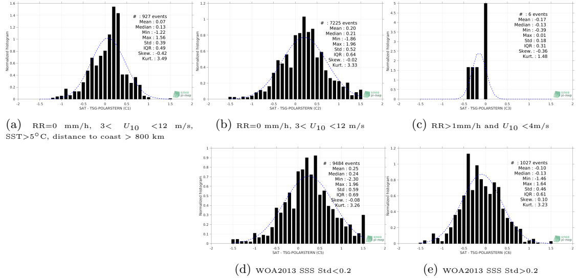
Figure 13: Normalized histogram of \Delta SSS (Aquarius-L2-OR-V5 - TSG-POLARSTERN) for 5 different subdatasets corresponding to: RR=0 mm/h, 3 < U_{10} < 12 m/s, SST>5°C, distance to coast > 800 km (a), RR=0 mm/h, 3 < U_{10} < 12 m/s (b), RR>1mm/h and U_{10} < 4 m/s (c), WOA2013 SSS Std<0.2 (d), WOA2013 SSS Std>0.2 (e).
