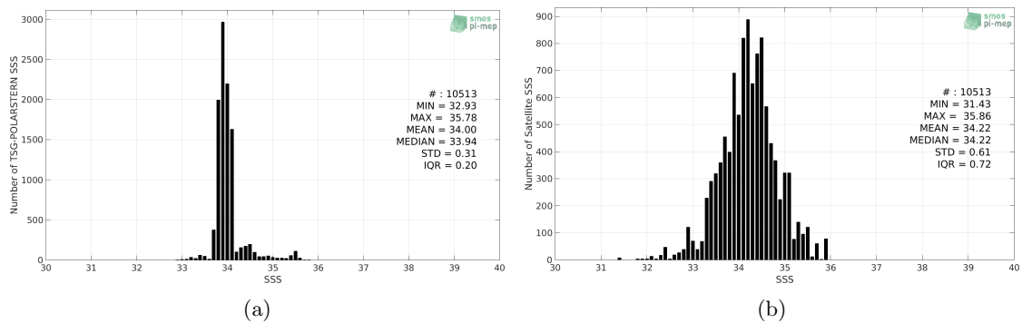
Figure 2: Histograms of SSS from TSG-POLARSTERN (a) and Aquarius-L2-OR-V5 (b) considering all match-up pairs per bins of 0.1 over the Roaring Forties and Furious Fifties Pi-MEP region and for the full satellite product period.
