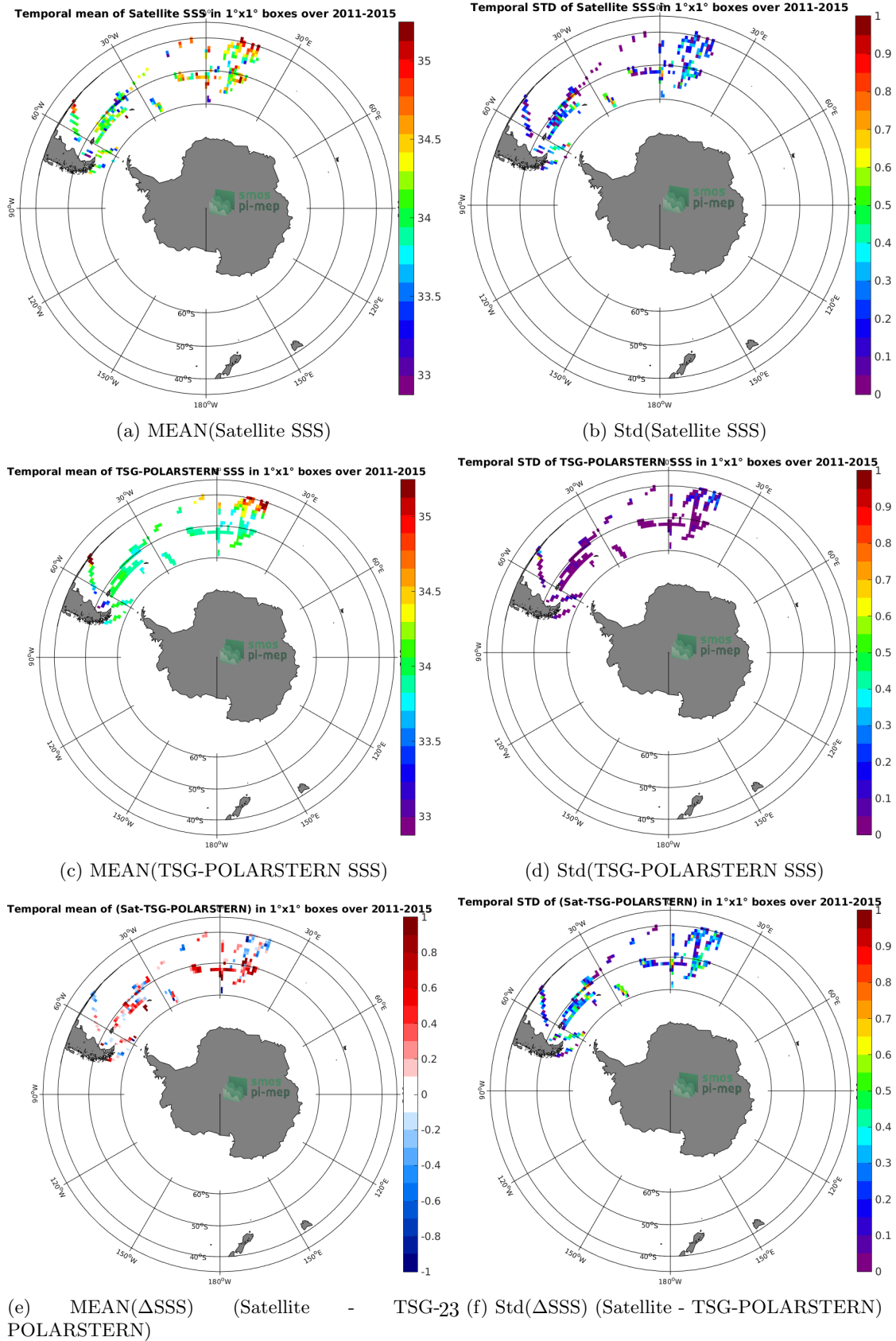
Figure 6: Temporal mean (left) and Std (right) of SSS from Aquarius-L2-OR-V5 (top), TSG-POLARSTERN (middle), and of \Delta SSS (Satellite - TSG-POLARSTERN). Only match-up pairs are used to generate these maps.
