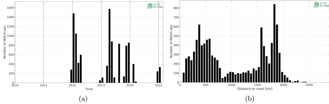
Figure 1: Number of match-ups between TSG-POLARSTERN and Aquarius-L2-OR-V5 SSS as a function of time (a) and as function of the distance to coast (b) over the Roaring Forties and Furious Fifties Pi-MEP region and for the full satellite product period.
