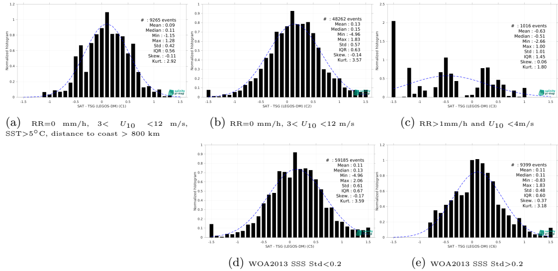
Figure 15: Normalized histogram of \Delta\text{SSS} (Aquarius SSS L2 OR v5 (NASA-GSFC) - TSG (LEGOS-DM)) for 5 different subdatasets corresponding to: RR=0 mm/h, 3 < U_{10} < 12 m/s, SST>5°C, distance to coast > 800 km (a), RR=0 mm/h, 3 < U_{10} < 12 m/s (b), RR>1mm/h and U_{10} < 4 m/s (c), WOA2013 SSS Std<0.2 (d), WOA2013 SSS Std>0.2 (e).
