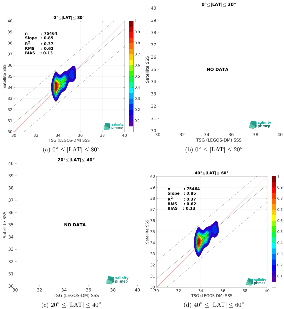
Figure 10: Contour maps of the concentration of Aquarius SSS L2 OR v5 (NASA-GSFC) SSS (y-axis) versus TSG (LEGOS-DM) SSS (x-axis) at match-up pairs for different latitude bands. For each plot, the red line shows x=y . The black thin and dashed lines indicate a linear fit through the data cloud and the \pm 95\% confidence levels, respectively. The number match-up pairs n , the slope and R^2 coefficient of the linear fit, the root mean square (RMS) and the mean bias between satellite and in situ data are indicated for each latitude band in each plot.
