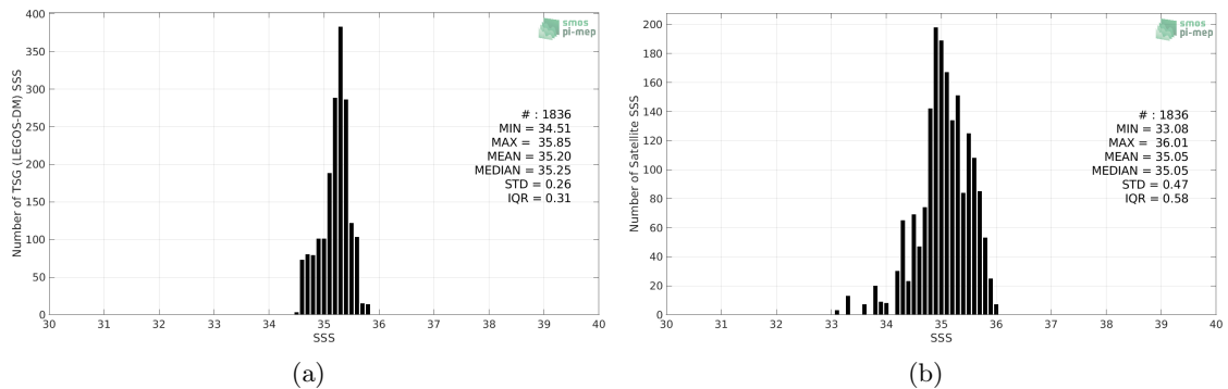
Figure 2: Histograms of SSS from TSG (LEGOS-DM) (a) and Aquarius SSS L2 OR v5 (NASA-GSFC) (b) considering all match-up pairs per bins of 0.1 over the Roaring Forties and Furious Fifties Pi-MEP region and for the full satellite product period.
