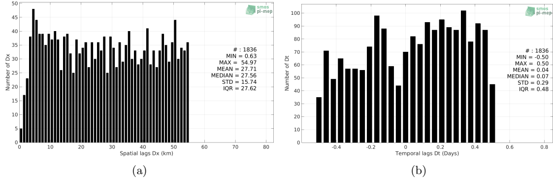
Figure 5: Histograms of the spatial (a) and temporal (b) lags between the time of the TSG (LEGOS-DM) measurements and the date of the corresponding Aquarius SSS L2 OR v5 (NASA-GSFC) SSS product.
