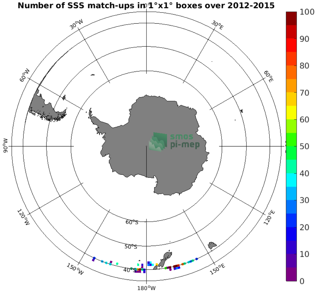
Figure 4: Number of SSS match-ups between TSG (LEGOS-DM) SSS and the Aquarius SSS L2 OR v5 (NASA-GSFC) SSS product for the Roaring Forties and Furious Fifties Pi-MEP region over 1°x1° boxes and for the full satellite product period.
