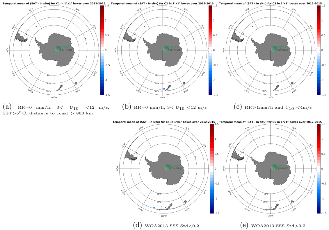
Figure 12: Temporal mean gridded over spatial boxes of size 1^{\circ}\times 1^{\circ} of \Delta\text{SSS} (Aquarius-L2-OR-V5 - TSG-LEGOS-DM) for 5 different subdatasets corresponding to:RR=0 mm/h, 3 < U_{10} < 12 m/s, SST >5^{\circ}\text{C} , distance to coast > 800 km (a), RR=0 mm/h, 3 < U_{10} < 12 m/s (b), RR >1 mm/h and U_{10} < 4 m/s (c), WOA2013 SSS Std <0.2 (d), WOA2013 SSS Std >0.2 (e).
