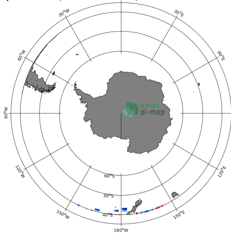
(e) MEAN( \Delta SSS) (Satellite - TSG-LEGOS-DM) 23
