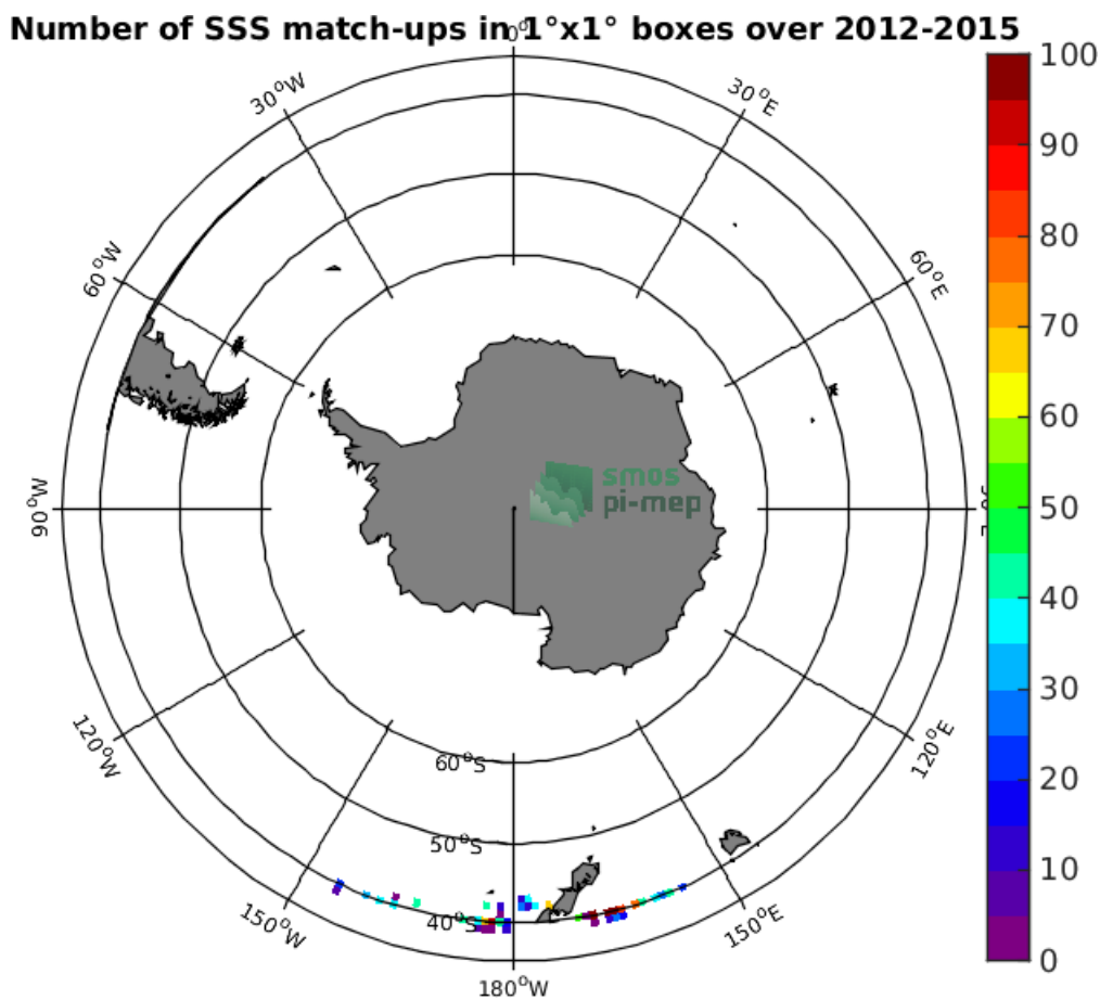
Figure 4: Number of SSS match-ups between TSG-LEGOS-DM SSS and the Aquarius-L2-OR-V5 SSS product for the Roaring Forties and Furious Fifties Pi-MEP region over 1^\circ \times 1^\circ boxes and for the full satellite product period.
