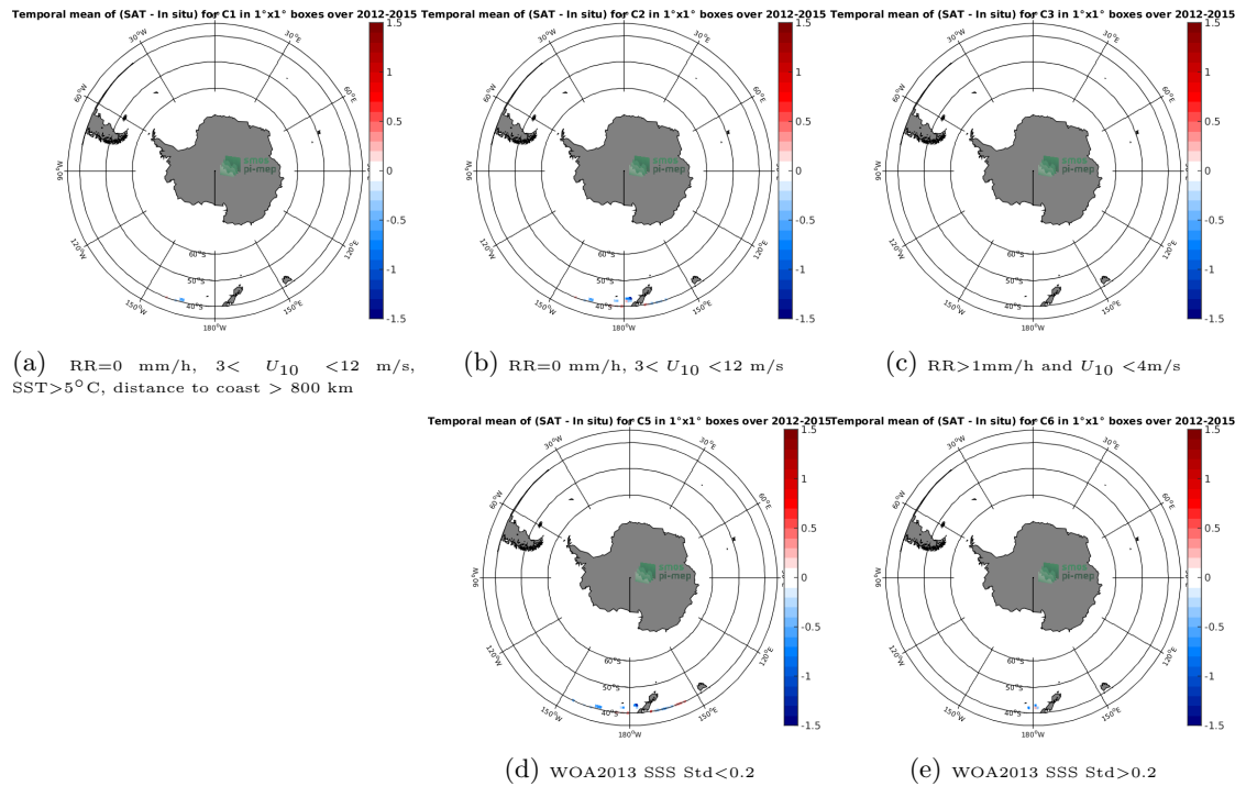
Figure 12: Temporal mean gridded over spatial boxes of size 1^\circ \times 1^\circ of \Delta SSS (Aquarius-L2-OR-V5 - TSG-LEGOS-DM) for 5 different subdatasets corresponding to:RR=0 mm/h, 3 < U_{10} < 12 m/s, SST > 5^\circ\text{C} , distance to coast > 800 km (a), RR=0 mm/h, 3 < U_{10} < 12 m/s (b), RR > 1 mm/h and U_{10} < 4 m/s (c), WOA2013 SSS Std < 0.2 (d), WOA2013 SSS Std > 0.2 (e).
