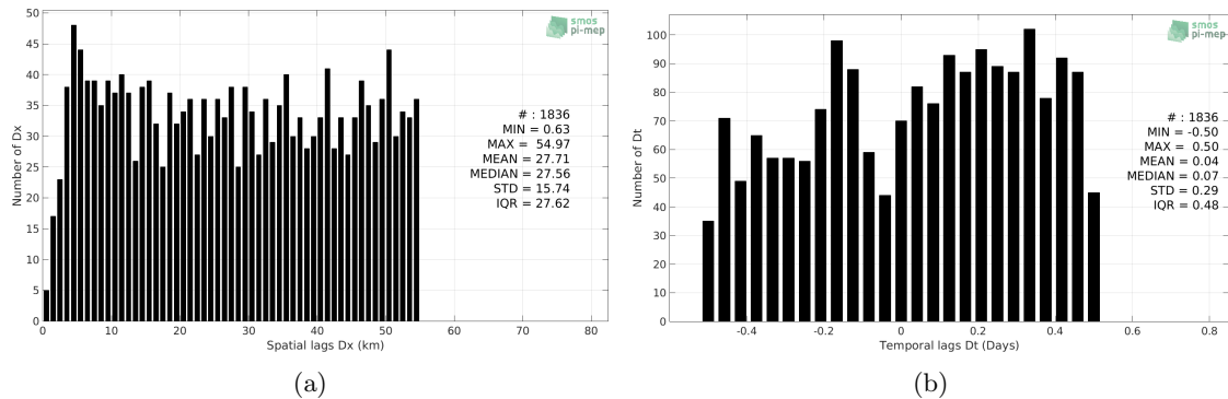
Figure 5: Histograms of the spatial (a) and temporal (b) lags between the time of the TSG-LEGOS-DM measurements and the date of the corresponding Aquarius-L2-OR-V5 SSS product.
