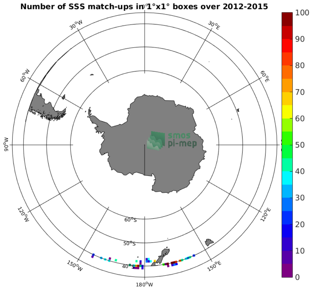
Figure 4: Number of SSS match-ups between TSG-LEGOS-DM SSS and the Aquarius-L2-OR-V5 SSS product for the Roaring Forties and Furious Fifties Pi-MEP region over 1°x1° boxes and for the full satellite product period.
