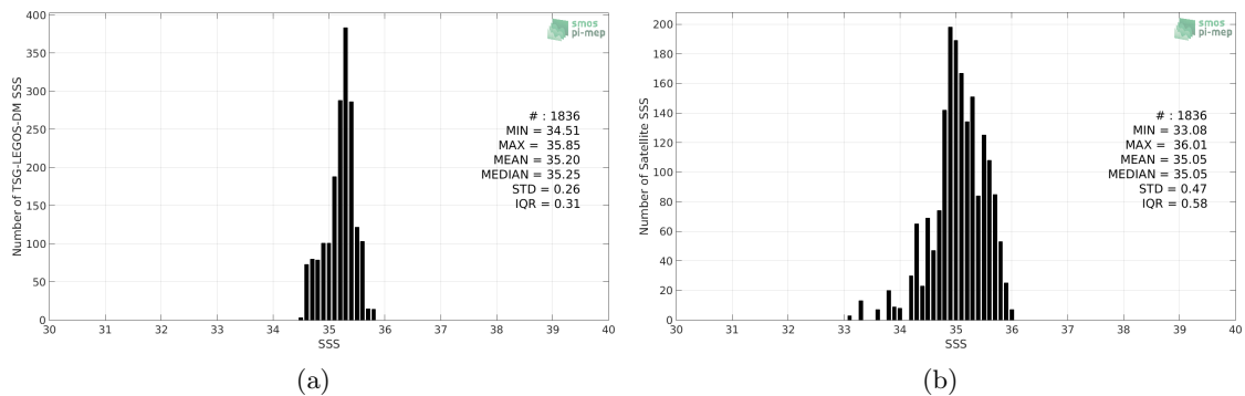
Figure 2: Histograms of SSS from TSG-LEGOS-DM (a) and Aquarius-L2-OR-V5 (b) considering all match-up pairs per bins of 0.1 over the Roaring Forties and Furious Fifties Pi-MEP region and for the full satellite product period.
