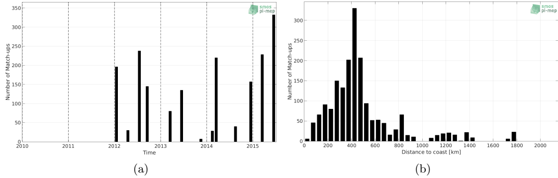
Figure 1: Number of match-ups between TSG-LEGOS-DM and Aquarius-L2-OR-V5 SSS as a function of time (a) and as function of the distance to coast (b) over the Roaring Forties and Furious Fifties Pi-MEP region and for the full satellite product period.
