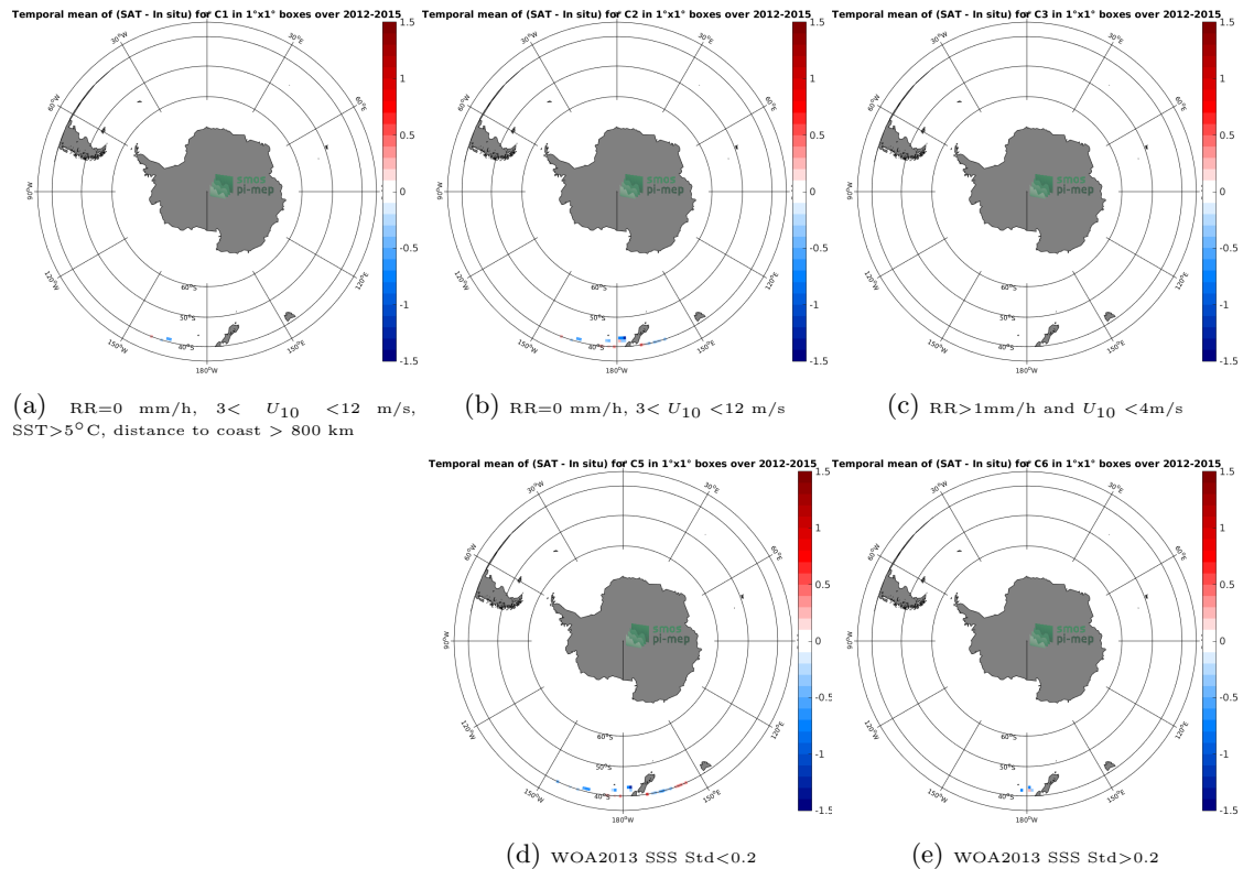
Figure 12: Temporal mean gridded over spatial boxes of size 1^\circ \times 1^\circ of \Delta SSS (Aquarius-L2-OR-V5 - TSG-LEGOS-DM) for 5 different subdatasets corresponding to:RR=0 mm/h, 3 < U_{10} < 12 m/s, SST >5^\circ C, distance to coast > 800 km (a), RR=0 mm/h, 3 < U_{10} < 12 m/s (b), RR >1 mm/h and U_{10} < 4 m/s (c), WOA2013 SSS Std <0.2 (d), WOA2013 SSS Std >0.2 (e).
