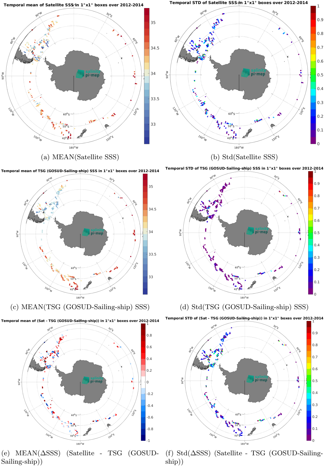
Figure 7: Temporal mean (left) and Std (right) of SSS from Aquarius SSS L2 OR v5 (NASA-GSFC) (top), TSG (GOSUD-Sailing-ship) (middle), and of \Delta SSS (Satellite - TSG (GOSUD-Sailing-ship)). Only match-up pairs are used to generate these maps.
