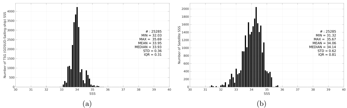
Figure 3: Histograms of SSS from TSG (GOSUD-Sailing-ship) (a) and Aquarius SSS L2 OR v5 (NASA-GSFC) (b) considering all match-up pairs per bins of 0.1 over the Roaring Forties and Furious Fifties Pi-MEP region and for the full satellite product period.
