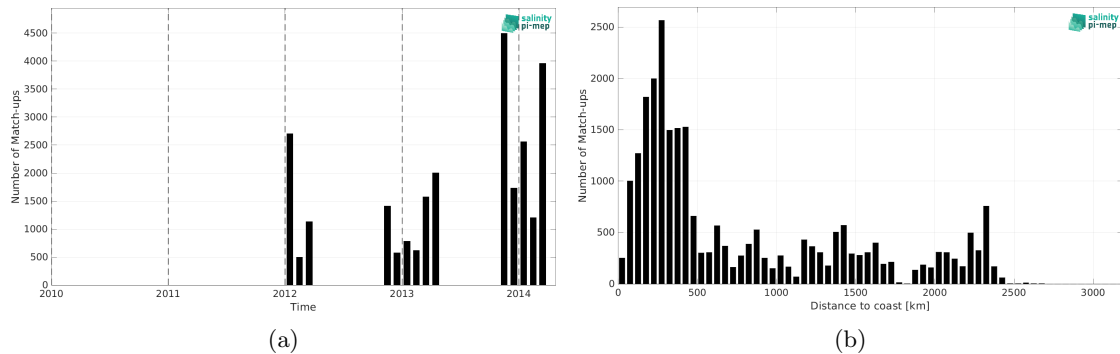
Figure 2: Number of match-ups between TSG (GOSUD-Sailing-ship) and Aquarius SSS L2 OR v5 (NASA-GSFC) SSS as a function of time (a) and as function of the distance to coast (b) over the Roaring Forties and Furious Fifties Pi-MEP region and for the full satellite product period.
