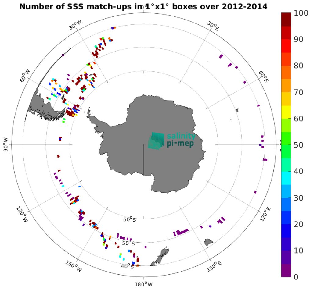
Figure 5: Number of SSS match-ups between TSG (GOSUD-Sailing-ship) SSS and the Aquarius SSS L2 OR v5 (NASA-GSFC) SSS product for the Roaring Forties and Furious Fifties Pi-MEP region over 1^\circ \times 1^\circ boxes and for the full satellite product period.
