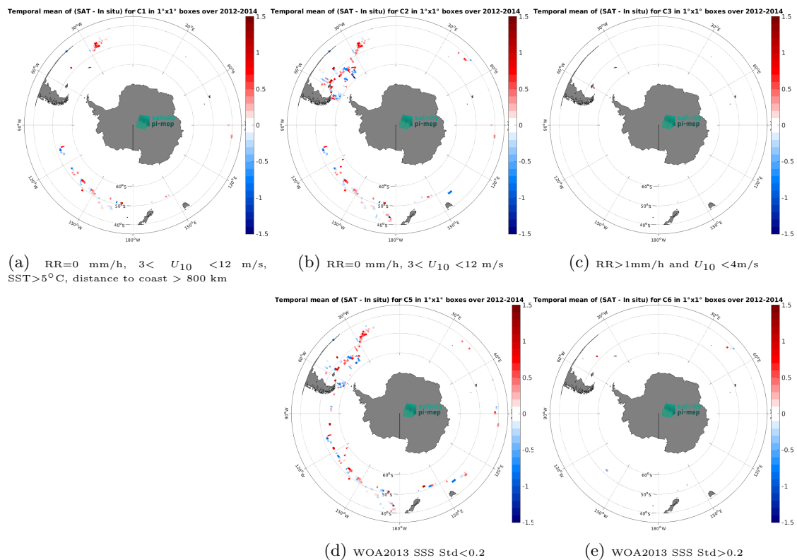
Figure 14: Temporal mean gridded over spatial boxes of size 1^\circ \times 1^\circ of \Delta SSS (Aquarius SSS L2 OR v5 (NASA-GSFC) - TSG (GOSUD-Sailing-ship)) for 5 different subdatasets corresponding to:RR=0 mm/h, 3 < U_{10} < 12 m/s, SST >5^\circ C, distance to coast > 800 km (a), RR=0 mm/h, 3 < U_{10} < 12 m/s (b), RR >1 mm/h and U_{10} < 4 m/s (c), WOA2013 SSS Std <0.2 (d), WOA2013 SSS Std >0.2 (e).
