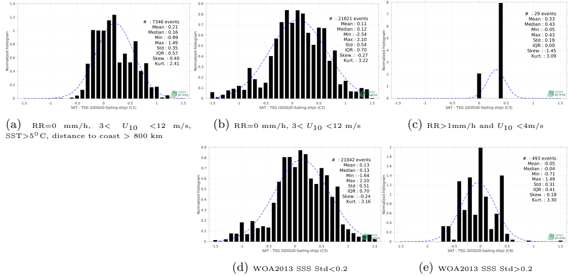
Figure 13: Normalized histogram of \Delta\text{SSS} (Aquarius SSS L2 OR v5 (NASA-GSFC) - TSG (GOSUD-Sailing-ship)) for 5 different subdatasets corresponding to: RR=0 mm/h, 3 < U_{10} < 12 m/s, SST > 5^\circ\text{C} , distance to coast > 800 km (a), RR=0 mm/h, 3 < U_{10} < 12 m/s (b), RR > 1\text{mm/h} and U_{10} < 4\text{m/s} (c), WOA2013 SSS Std < 0.2 (d), WOA2013 SSS Std > 0.2 (e).
