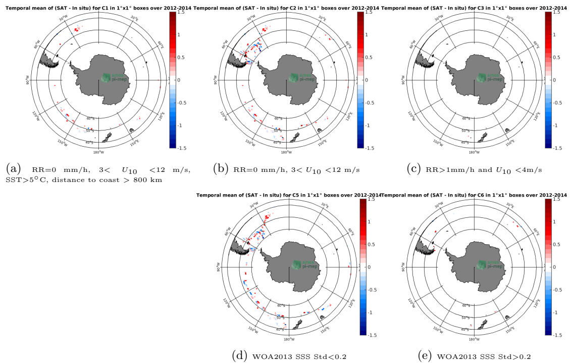
Figure 12: Temporal mean gridded over spatial boxes of size 1^\circ \times 1^\circ of \Delta SSS (Aquarius-L2-OR-V5 - TSG-GOSUD-Sailing-ship) for 5 different subdatasets corresponding to:RR=0 mm/h, 3 < U_{10} < 12 m/s, SST >5^\circ C, distance to coast > 800 km (a), RR=0 mm/h, 3 < U_{10} < 12 m/s (b), RR >1 mm/h and U_{10} < 4 m/s (c), WOA2013 SSS Std <0.2 (d), WOA2013 SSS Std >0.2 (e).
