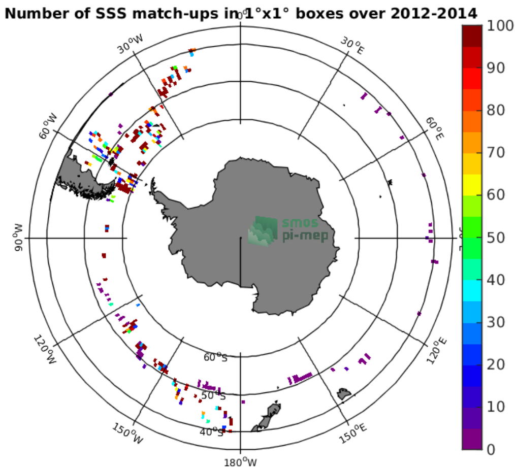
Figure 4: Number of SSS match-ups between TSG-GOSUD-Sailing-ship SSS and the Aquarius-L2-OR-V5 SSS product for the Roaring Forties and Furious Fifties Pi-MEP region over 1°x1° boxes and for the full satellite product period.
