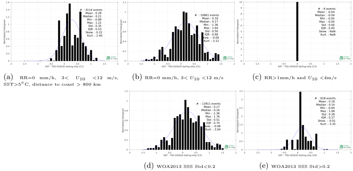
Figure 13: Normalized histogram of \Delta SSS (Aquarius-L2-OR-V5 - TSG-GOSUD-Sailing-ship) for 5 different subdatasets corresponding to: RR=0 mm/h, 3 < U_{10} < 12 m/s, SST > 5°C, distance to coast > 800 km (a), RR=0 mm/h, 3 < U_{10} < 12 m/s (b), RR > 1mm/h and U_{10} < 4 m/s (c), WOA2013 SSS Std < 0.2 (d), WOA2013 SSS Std > 0.2 (e).
