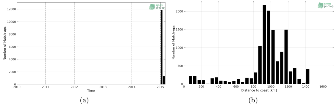
Figure 1: Number of match-ups between TSG (GOSUD-Research-vessel) and Aquarius SSS L2 OR v5 (NASA-GSFC) SSS as a function of time (a) and as function of the distance to coast (b) over the Roaring Forties and Furious Fifties Pi-MEP region and for the full satellite product period.
