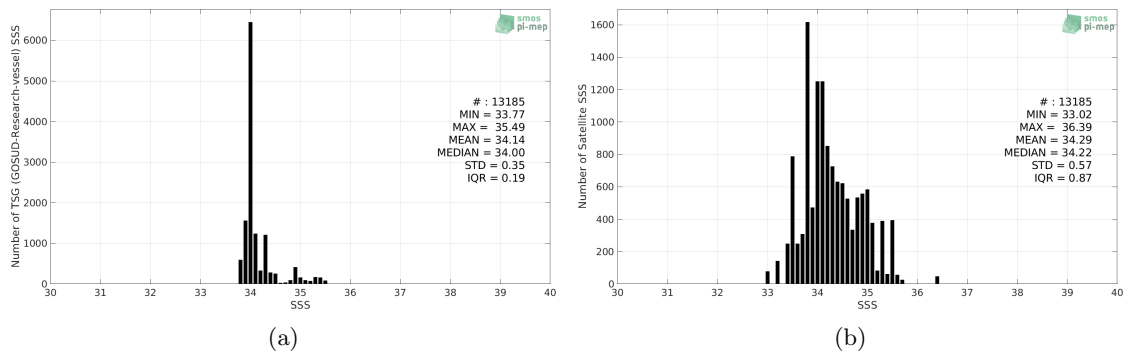
Figure 2: Histograms of SSS from TSG (GOSUD-Research-vessel) (a) and Aquarius SSS L2 OR v5 (NASA-GSFC) (b) considering all match-up pairs per bins of 0.1 over the Roaring Forties and Furious Fifties Pi-MEP region and for the full satellite product period.
