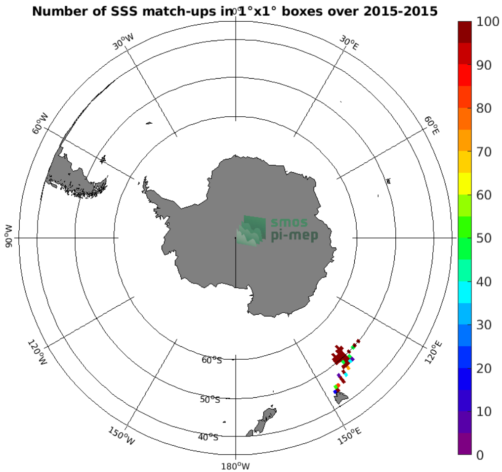
Figure 4: Number of SSS match-ups between TSG (GOSUD-Research-vessel) SSS and the Aquarius SSS L2 OR v5 (NASA-GSFC) SSS product for the Roaring Forties and Furious Fifties Pi-MEP region over 1^\circ \times 1^\circ boxes and for the full satellite product period.
