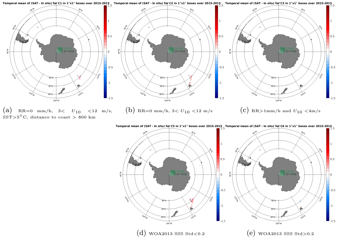
Figure 12: Temporal mean gridded over spatial boxes of size 1°x1° of \Delta SSS (Aquarius SSS L2 OR v5 (NASA-GSFC) - TSG (GOSUD-Research-vessel)) for 5 different subdatasets corresponding to:RR=0 mm/h, 3 < U_{10} < 12 m/s, SST>5°C, distance to coast > 800 km (a), RR=0 mm/h, 3 < U_{10} < 12 m/s (b), RR>1mm/h and U_{10} < 4 m/s (c), WOA2013 SSS Std<0.2 (d), WOA2013 SSS Std>0.2 (e).
