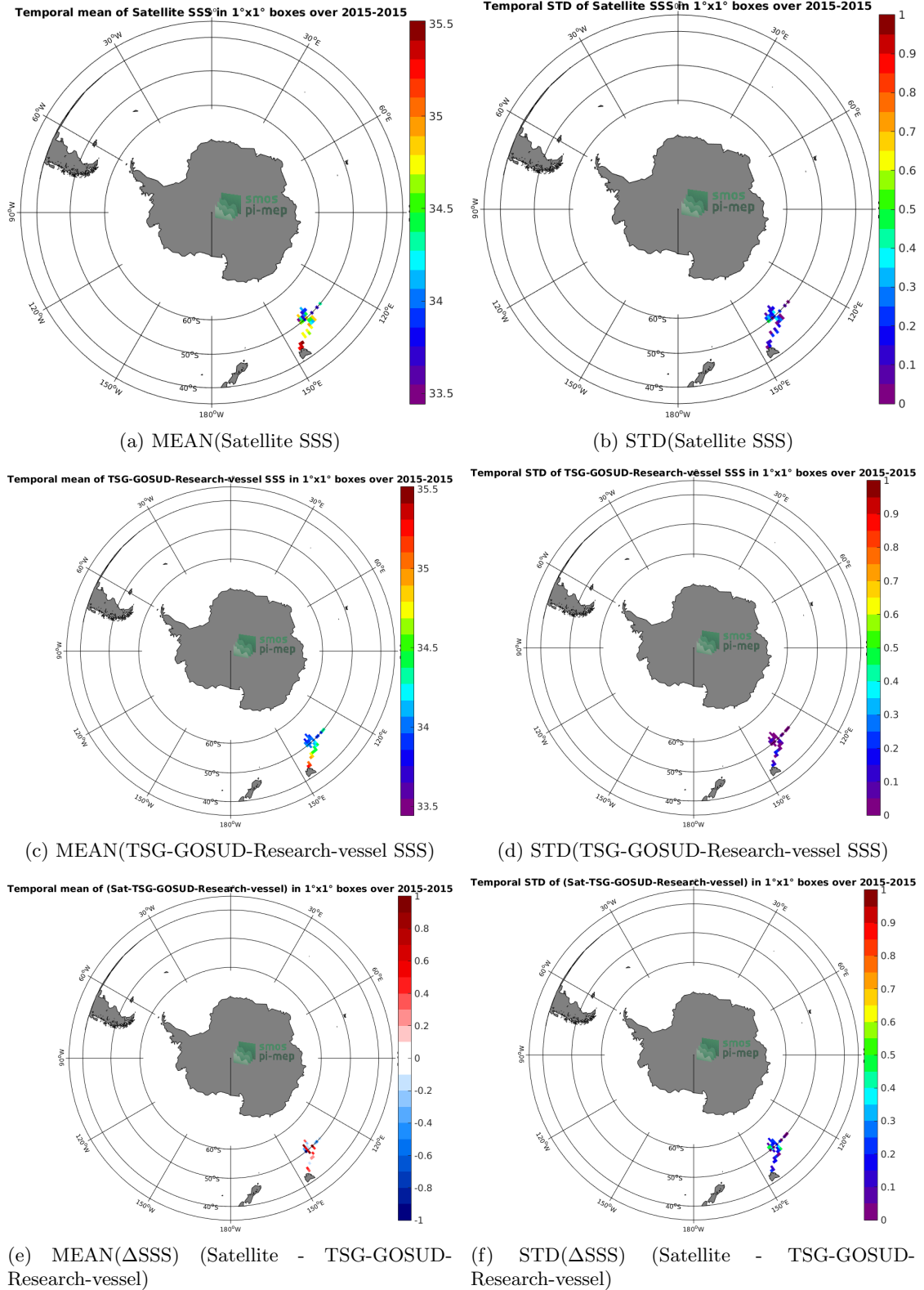
Figure 6: Temporal mean (left) and STD (right) of SSS from Aquarius-L2-OR-V5 (top), TSG-GOSUD-Research-vessel (middle), and of \Delta SSS 16 (Satellite - TSG-GOSUD-Research-vessel). Only match-up pairs are used to generate these maps.
