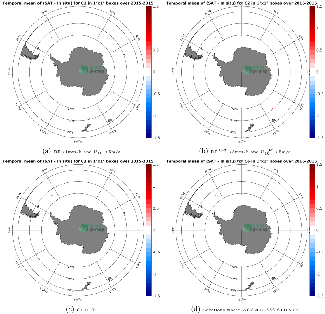
Figure 12: Temporal mean gridded over spatial boxes of size 1^\circ \times 1^\circ of \Delta SSS (Aquarius-L2-OR-V5 - TSG-GOSUD-Research-vessel) for 4 different subdatasets corresponding to: RR > 1mm/h and U_{10} < 5 m/s (a), RR^{10d} > 5 mm/h and U_{10}^{10d} < 5 m/s (b), C1 U C2 (c), Locations where WOA2013 SSS STD > 0.2 (d).
